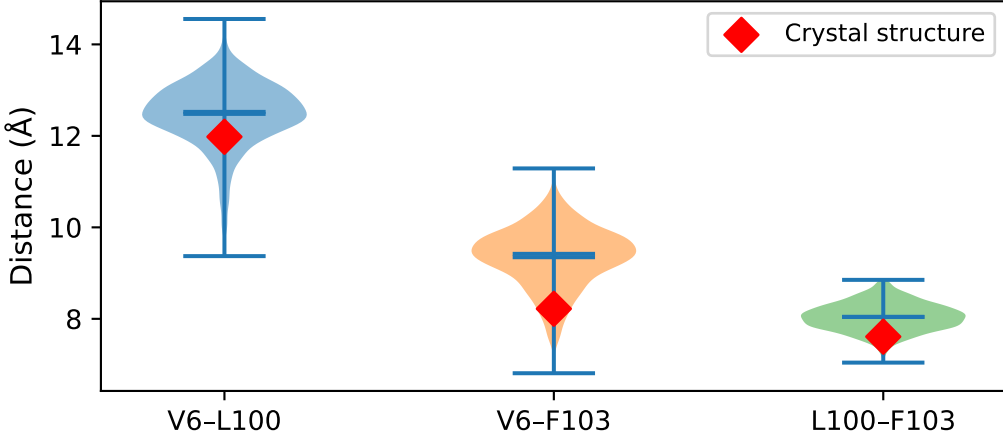
(E) Distance Distributions
