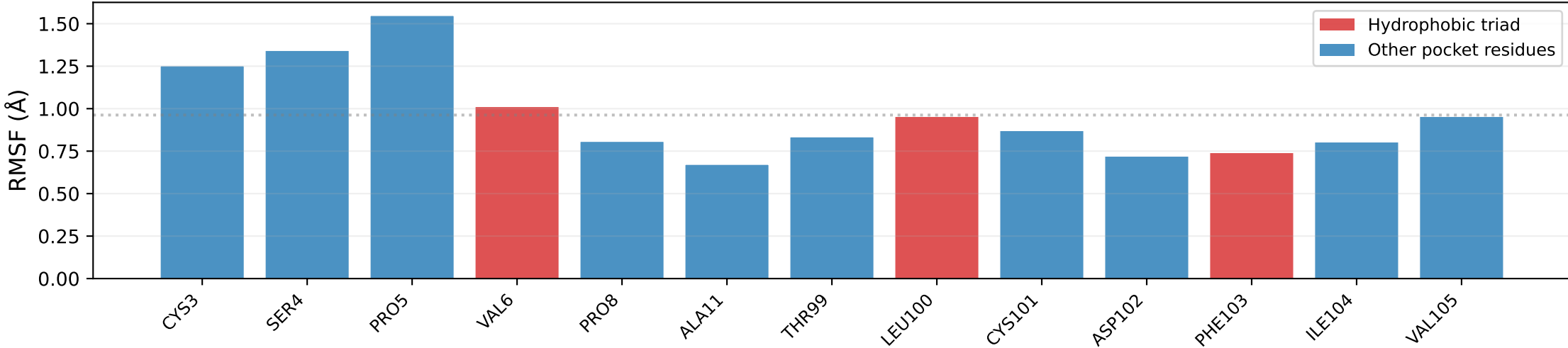
(C) Per-Residue Cα RMSF — Site 1 Pocket
