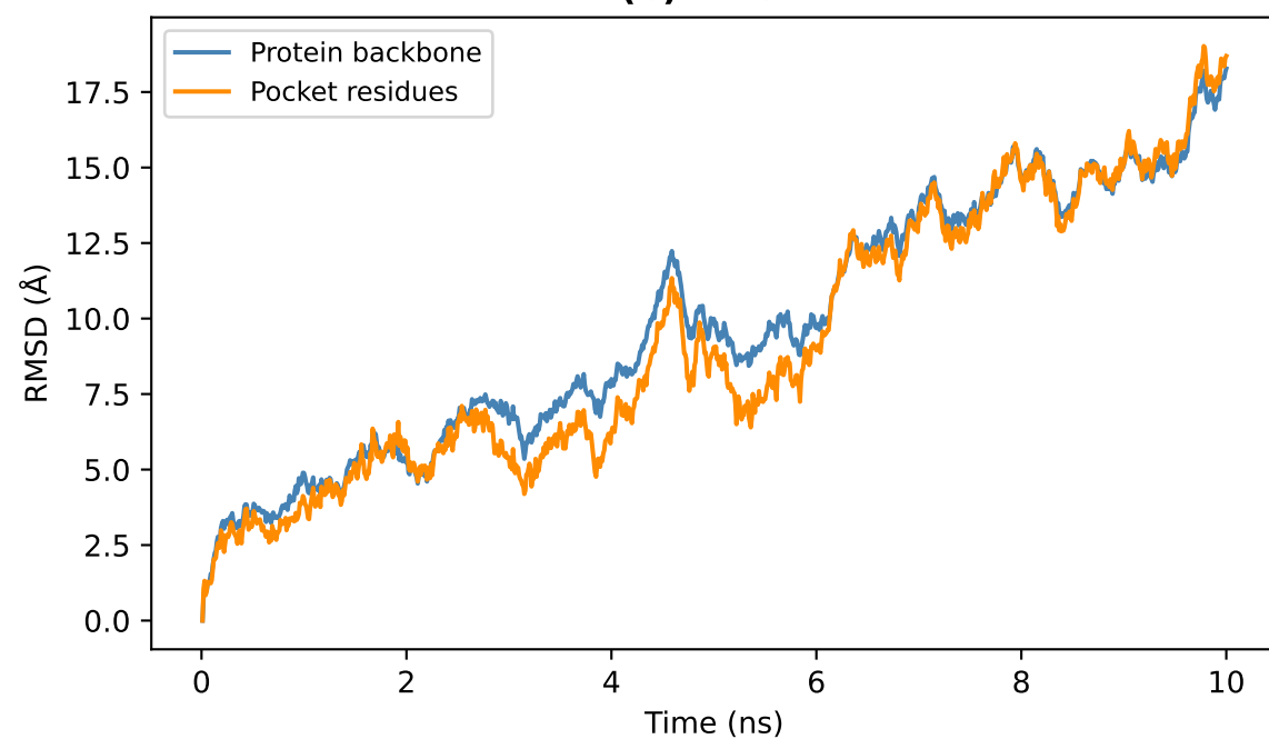
(C) RMSD
