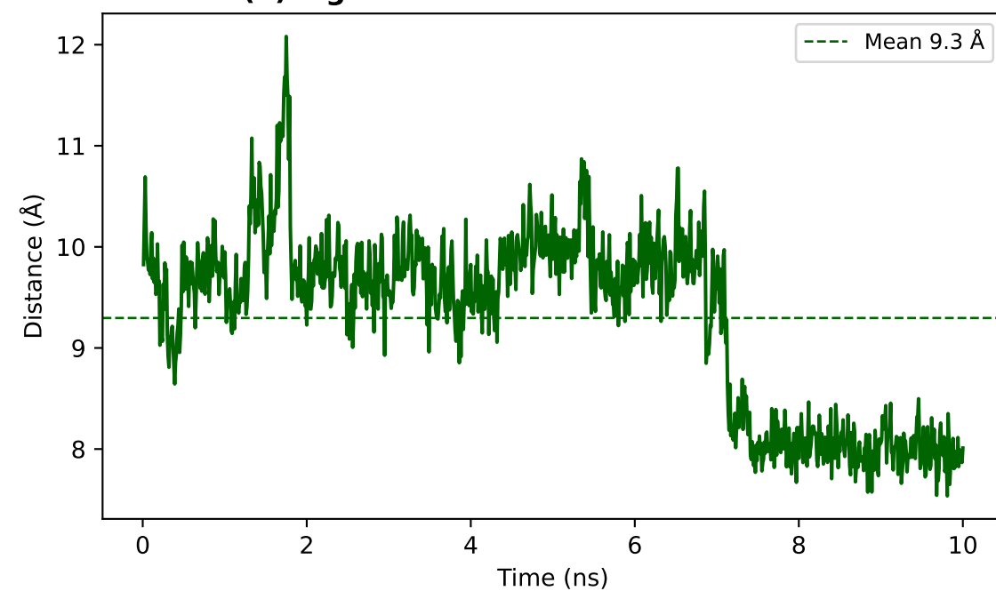
(F) Ligand COM - Pocket COM Distance
