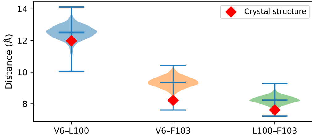
(E) Distance Distributions
