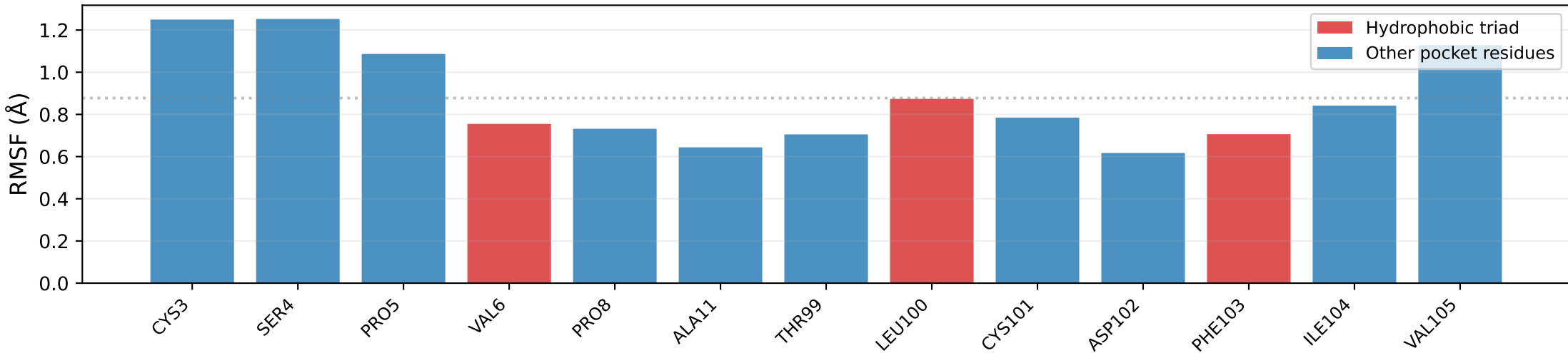
(C) Per-Residue Cα RMSF — Site 1 Pocket
