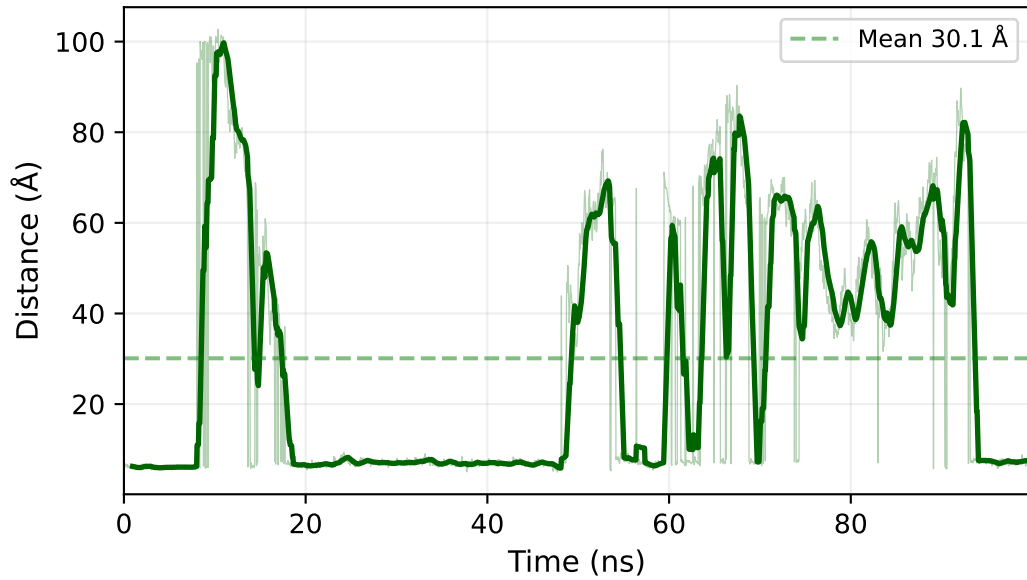
(G) Ligand COM - Pocket COM Distance
