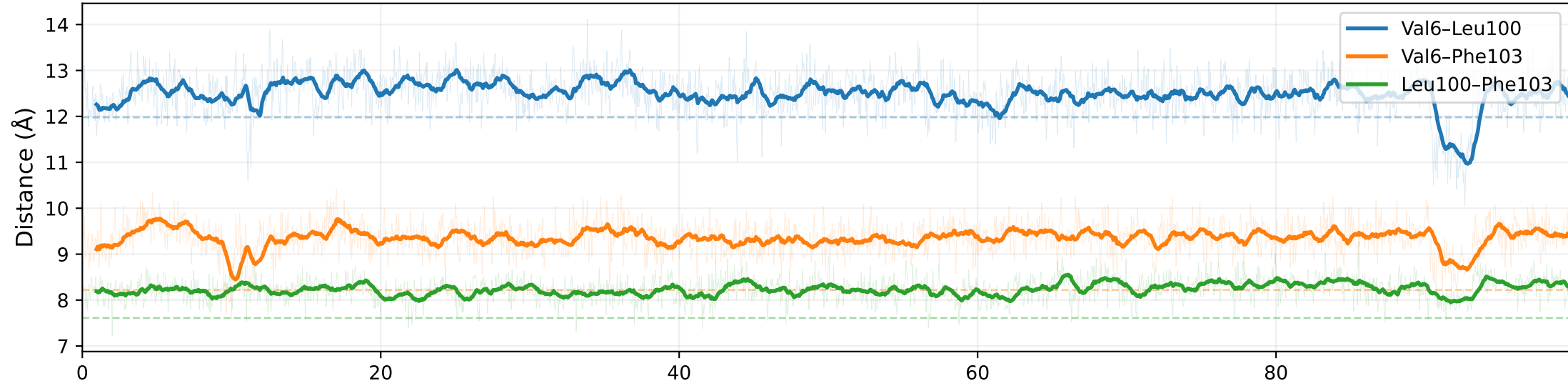
(A) Hydrophobic Triad Cα Distances
