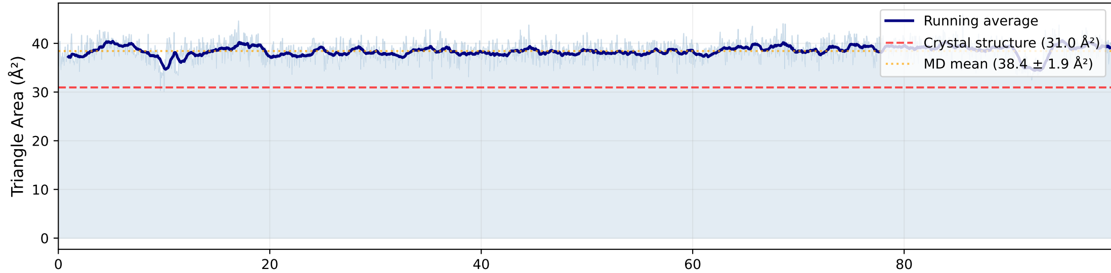
(B) Pocket Openness (Triad Triangle Area)
