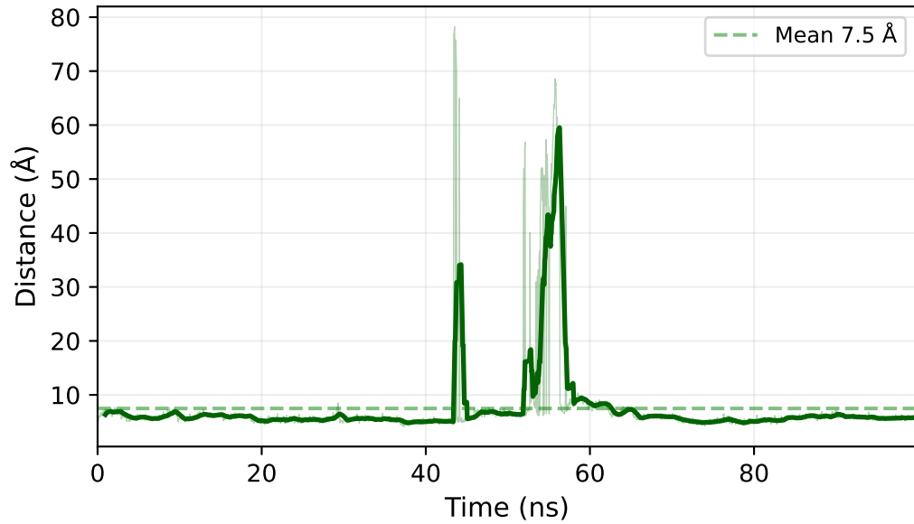
(G) Ligand COM - Pocket COM Distance
