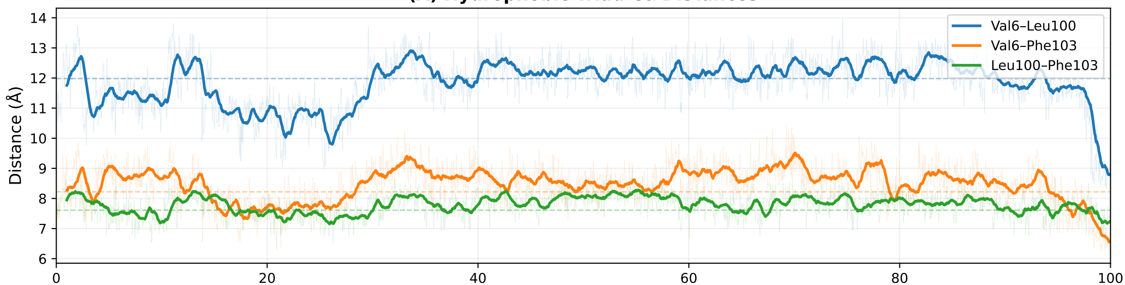
(A) Hydrophobic Triad C \alpha Distances
