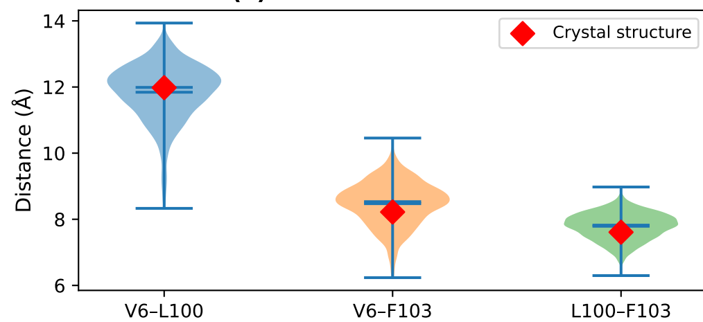
(E) Distance Distributions
