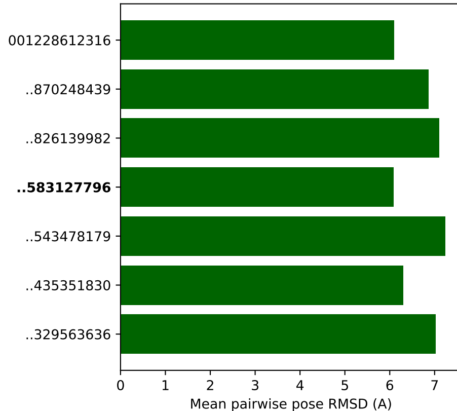
(B) Pose convergence (lower = tighter)
