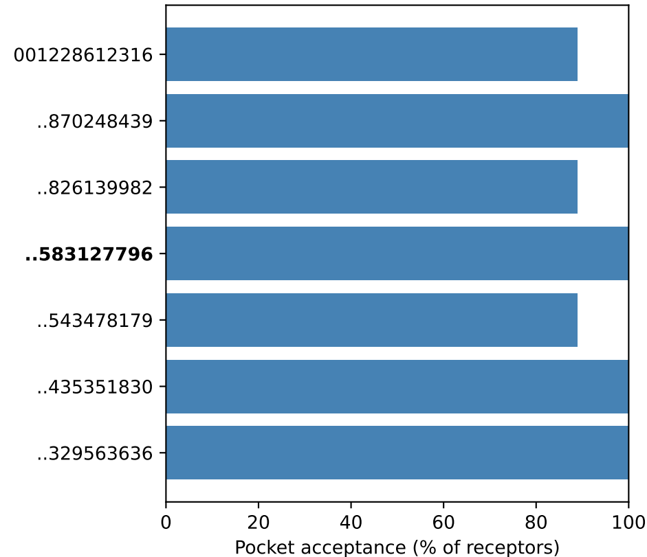
(A) Site 1 acceptance across ensemble
