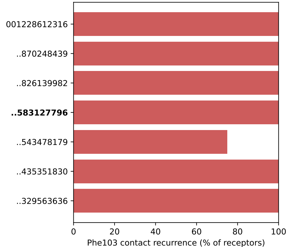
(C) Phe103 anchor recurrence
