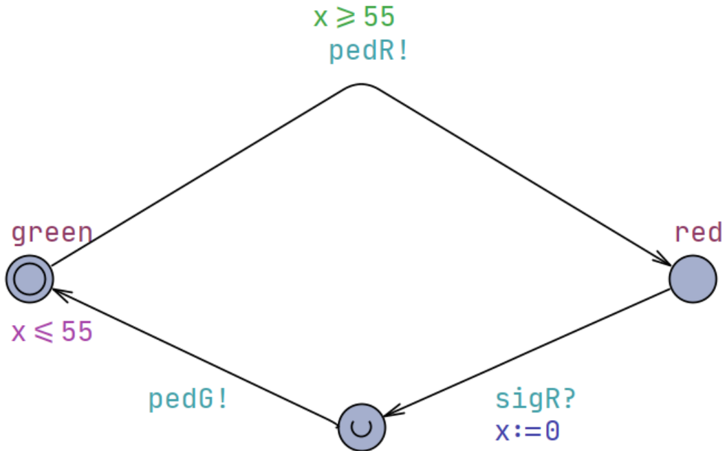
Figure 7: Crosswalk / pedestrian-side signal system (B.2).
