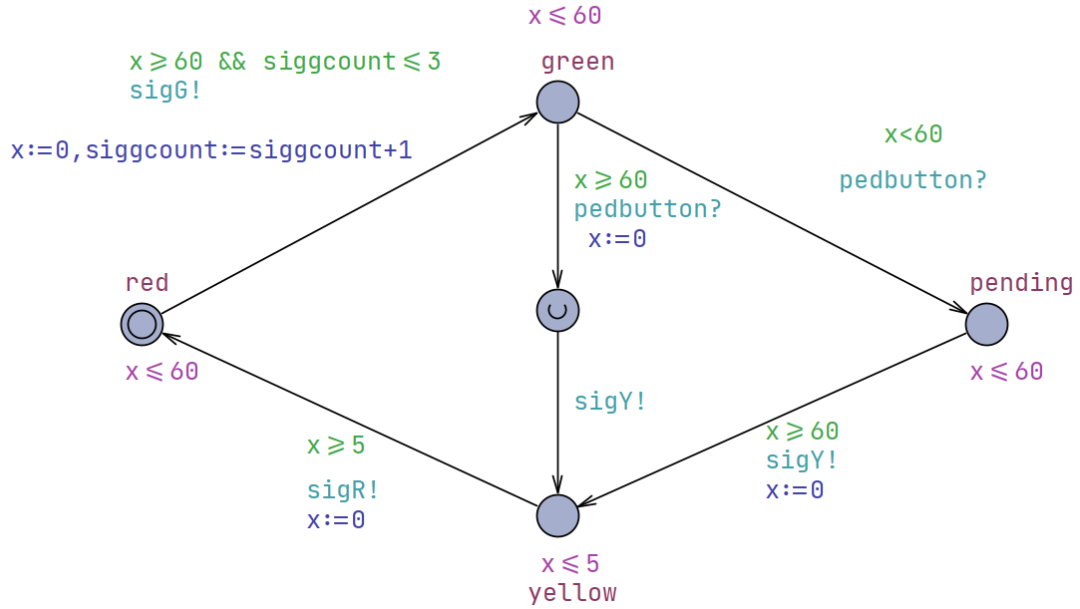
Figure 6: Timed automata for the traffic-light system (B.2).
