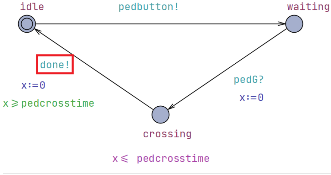
Figure 16: Pedestrian model cooperating with done (B.5).
