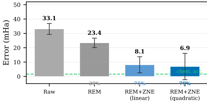
LiH mitigation ladder ( R = 1.6 \text{ \AA} )
