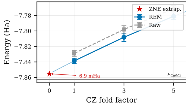
Richardson extrapolation
