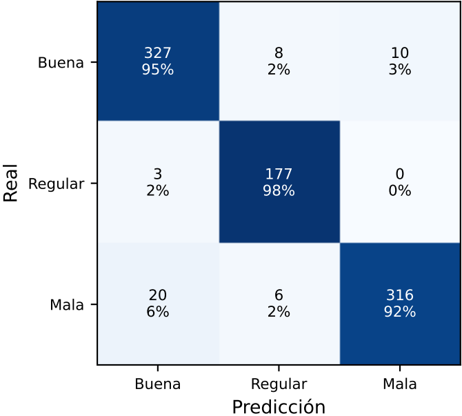
CNN (acc=94.6%)
