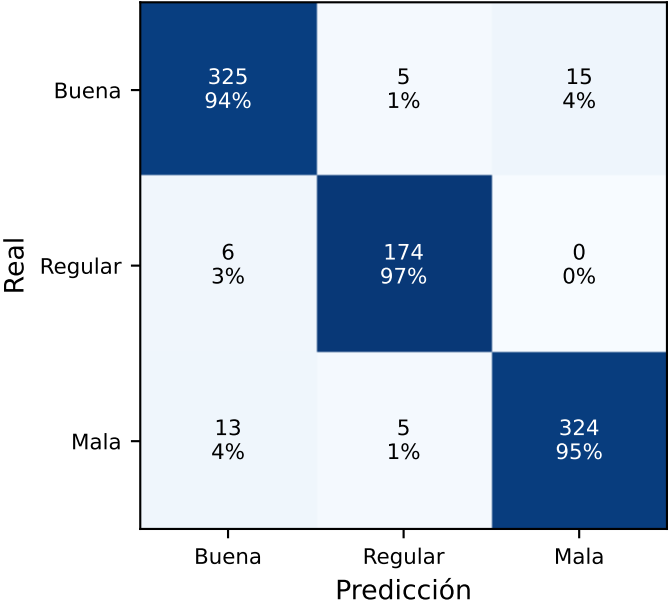
RandomForest (acc=94.9%)
