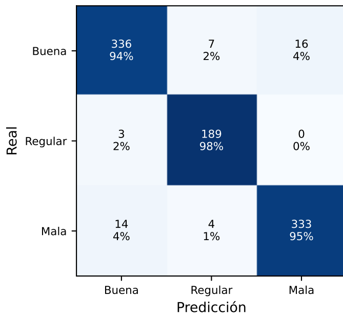
CNN (acc=95.1%)
