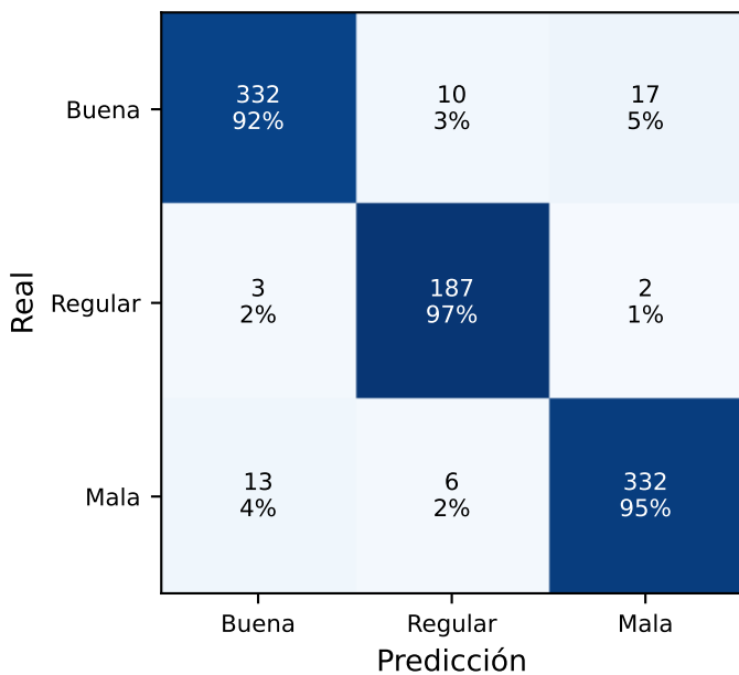
RandomForest (acc=94.3%)
