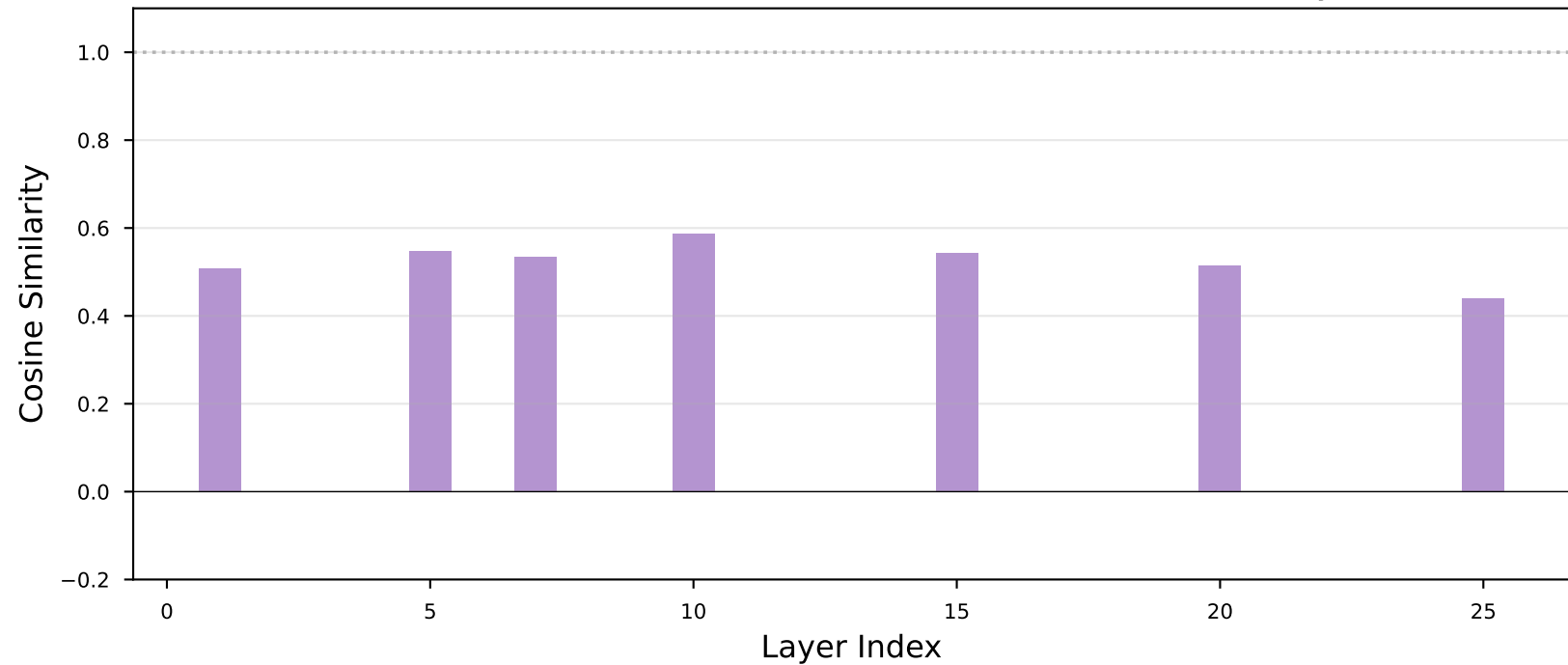
Probe Direction vs. Refusal Direction (Cosine Similarity)
