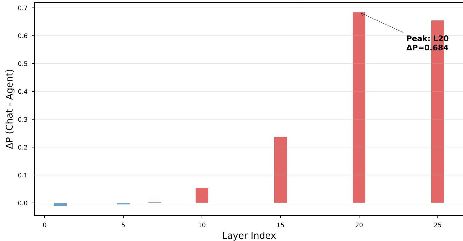
Projection Gap by Layer
