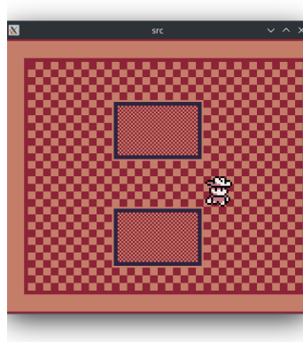
Figure 4: Day Mode
