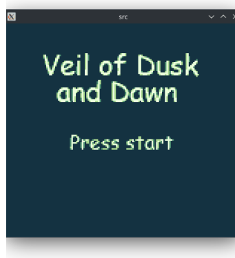
Figure 2: Title Screen
