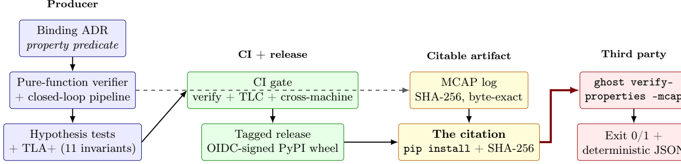
Figure 1: The safety citation pattern (C1). A binding ADR states the property predicate; a pure-function verifier and TLA+ specs encode its semantics; CI gates every push and tagging cuts an OIDC-signed release. The citable artifact is the pair (MCAP SHA-256, PyPI version). A third party concatenates them with one shell command and obtains a deterministic JSON verdict per property. The contribution of this paper is the assembly of the seven boxes into one shippable unit; the property set, the closed-form bound and the TLA+ specs instantiate the pattern on a representative supervisor.
