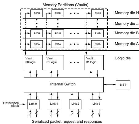
Figure 1. An Example Implementation of HMC.
