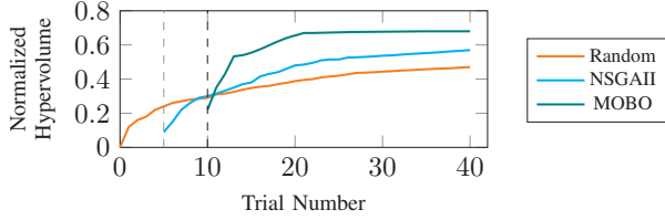
Fig. 10: Normalized hypervolume improvements of random search, NSGAIL, and MOBO.
