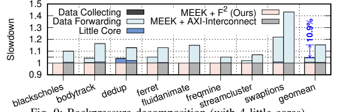
Fig. 9: Backpressure decomposition (with 4 little cores).
