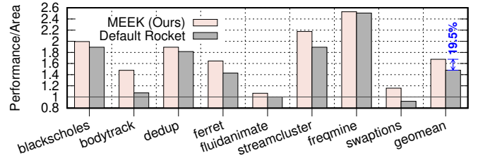
Fig. 10: Performance-area analysis of the little core.
