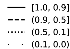
Success Rate
