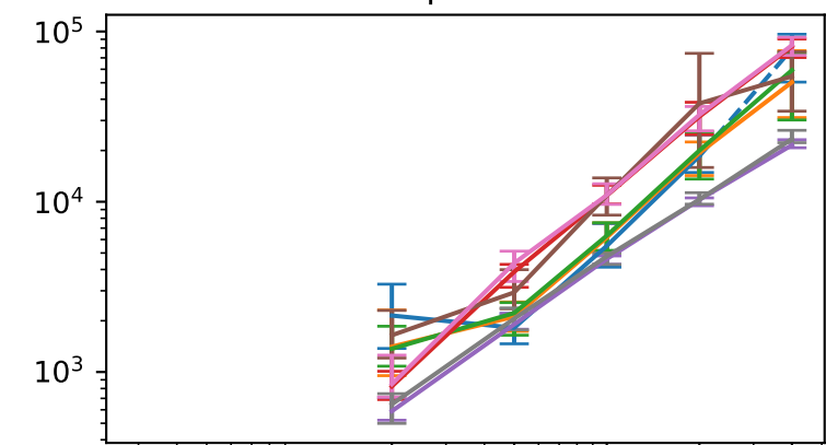
Sphere
