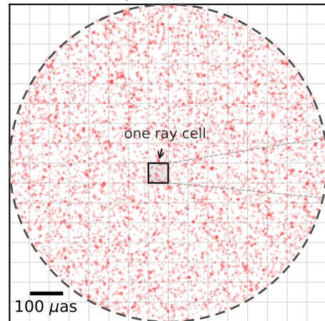
Partition lens plane into 16 \times 16 cells
