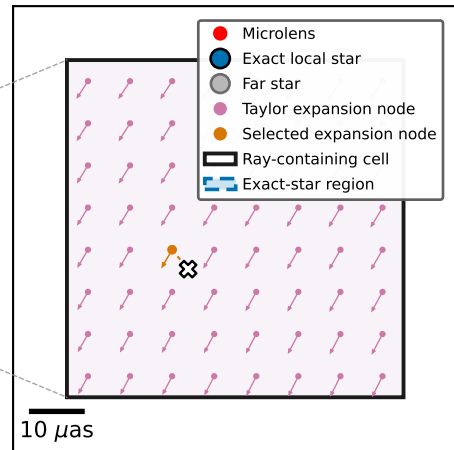
Evaluate order-4 Taylor far-field deflection
