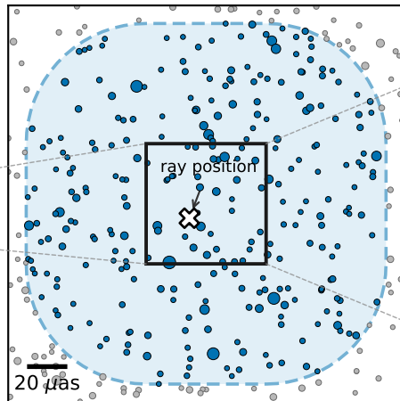
Sum nearby stars exactly
