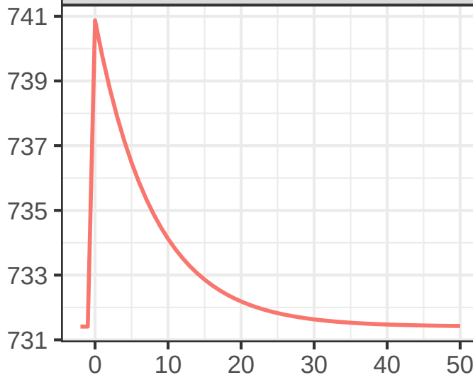
CH4_concentration (ppbv CH4)
