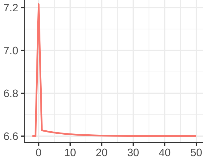
RF_H2O_strat (W/m2)
