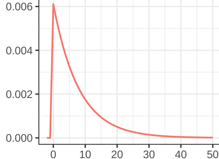
global_tas (degC)
