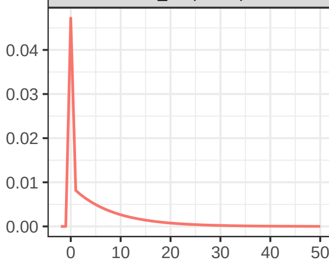
RF_tot (W/m2)
