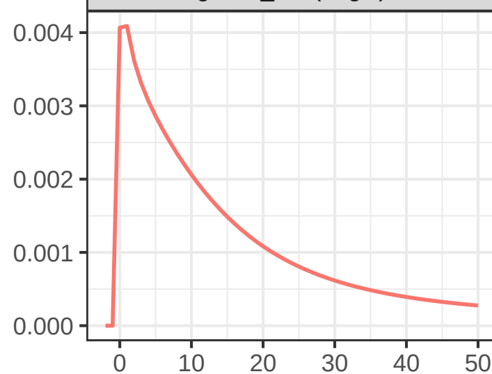
global_tas (degC)
