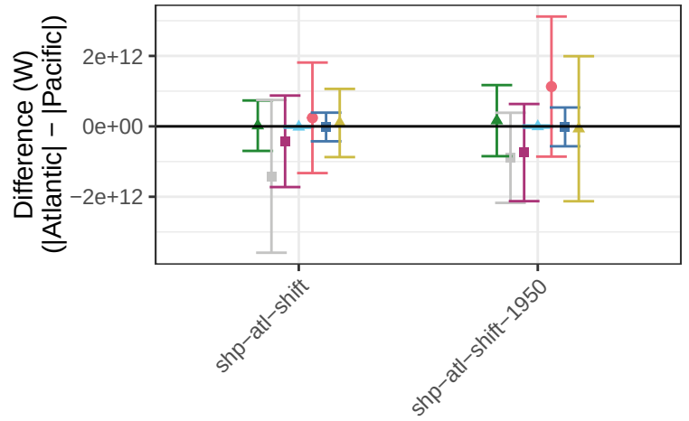
Clear-Sky Upwelling Longwave Flux – Difference Between Atlantic and Pacific
