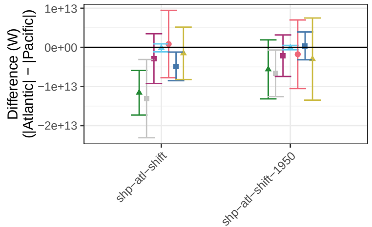
Implied Cloud Response – Difference Between Atlantic and Pacific
