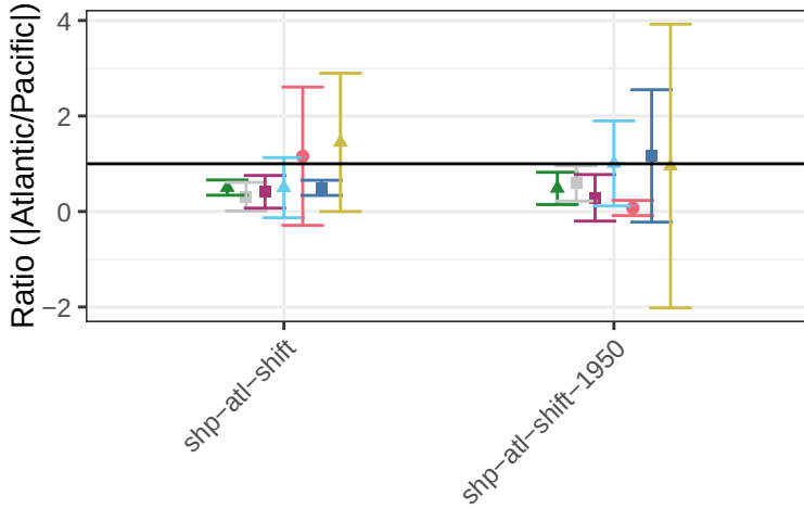
Upwelling Shortwave Flux – Ratio Between Atlantic and Pacific
