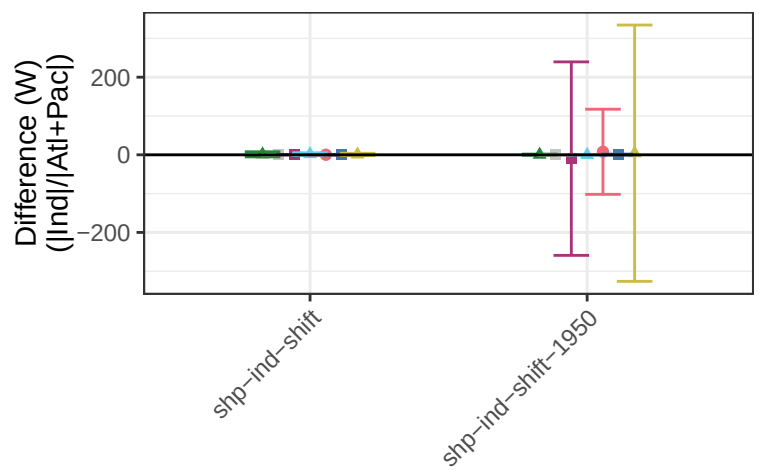
Clear-Sky Upwelling Longwave Flux – Ratio Between Ind and Atl+Pac
