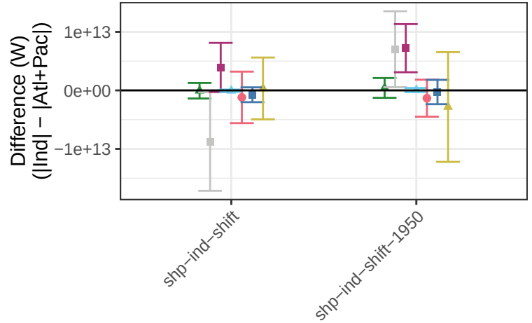
Upwelling Longwave Flux – Difference Between Ind and Atl+Pac
