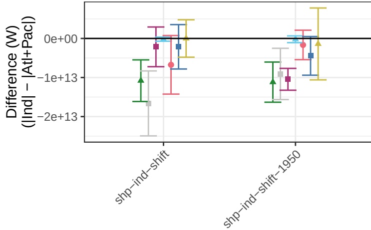
Upwelling Shortwave Flux – Difference Between Ind and Atl+Pac
