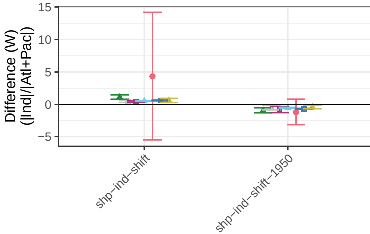
Clear-Sky Upwelling Shortwave Flux – Ratio Between Ind and Atl+Pac
