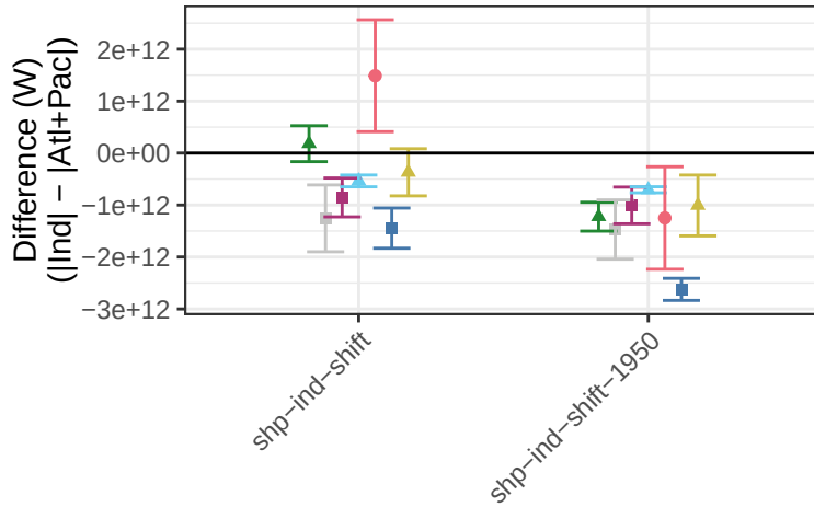
Clear-Sky Upwelling Shortwave Flux – Difference Between Ind and Atl+Pac
