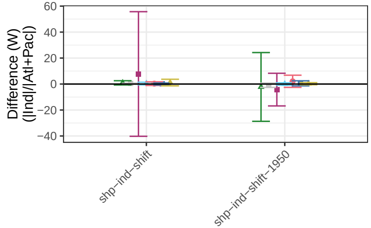
Upwelling Longwave Flux – Ratio Between Ind and Atl+Pac
