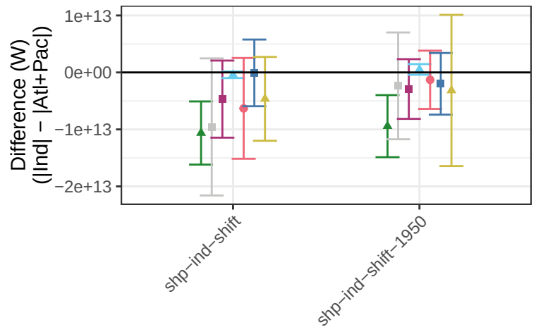
Implied Cloud Response – Difference Between Ind and Atl+Pac
