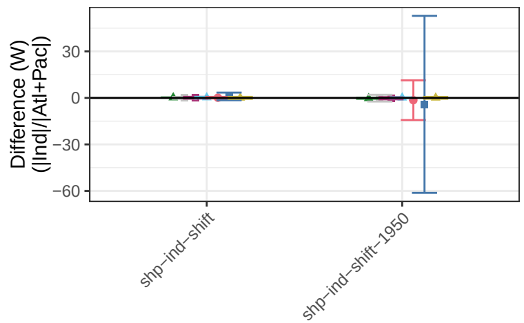
Implied Cloud Response – Ratio Between Ind and Atl+Pac
