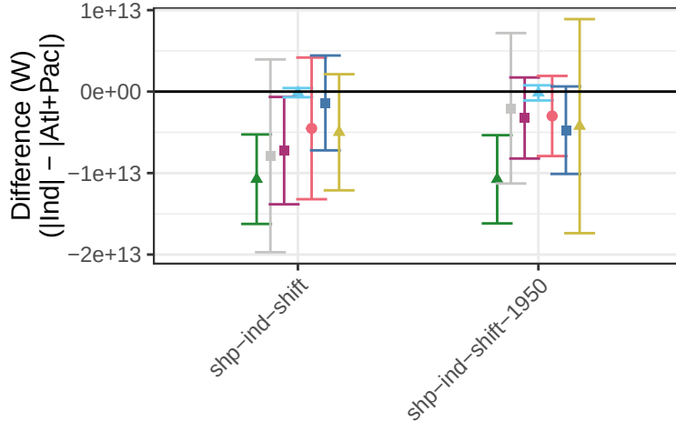
Net Radiative Flux – Difference Between Ind and Atl+Pac
