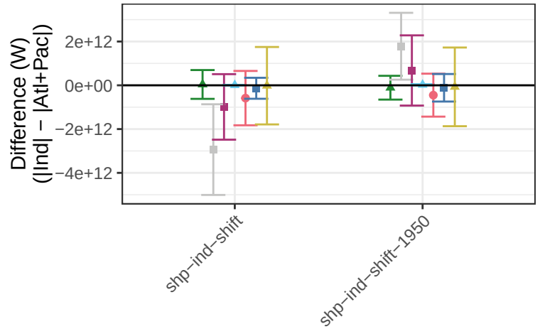
Clear-Sky Upwelling Longwave Flux – Difference Between Ind and Atl+Pac
