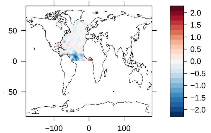
Upwelling Longwave Radiation at TOA ( \text{W/m}^2 ) – CESM1
