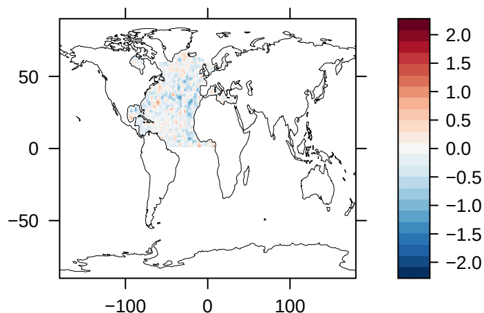
Clear-Sky Upwelling Longwave Radiation at TOA ( \text{W/m}^2 ) – CAM-ATRAS
