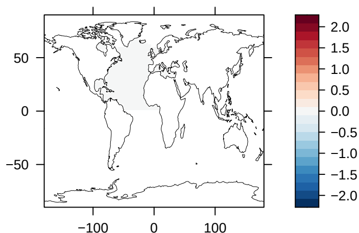
Clear-Sky Upwelling Longwave Radiation at TOA (W/m 2 ) – CAM-ATRAS
