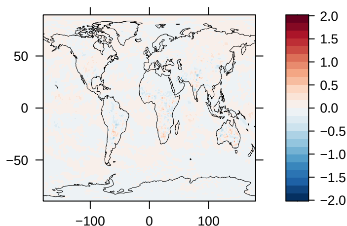
Clear-Sky Upwelling Longwave Radiation at TOA ( \text{W/m}^2 ) – GFDL-ESM4
