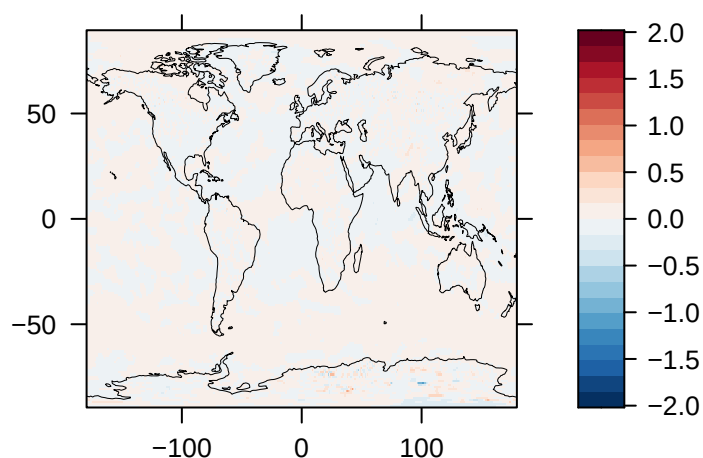
Clear-Sky Upwelling Longwave Radiation at TOA ( \text{W/m}^2 ) – E3SM
