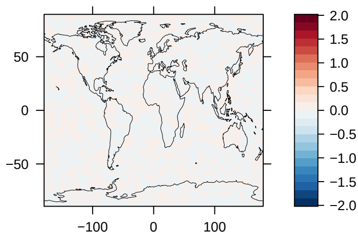
Clear-Sky Upwelling Longwave Radiation at TOA ( \text{W/m}^2 ) – GISS-E2.1
