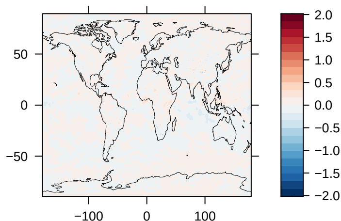
Clear-Sky Upwelling Longwave Radiation at TOA ( \text{W/m}^2 ) – NorESM2
