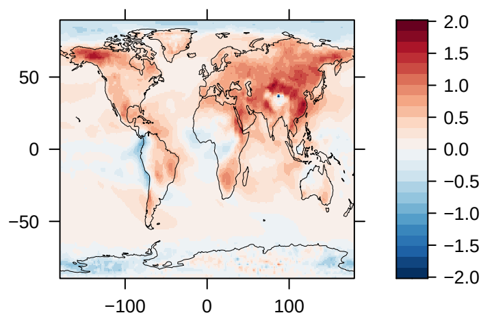
Clear-Sky Upwelling Longwave Radiation at TOA ( \text{W/m}^2 ) – CESM1
