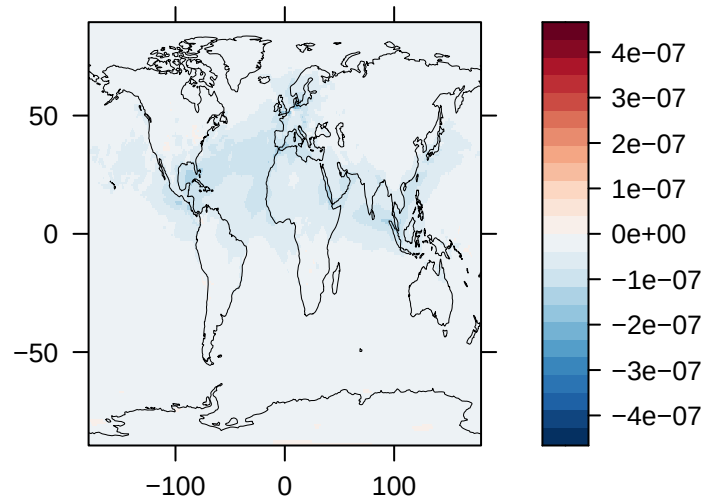
Load of SO 4 (% Diff) – GFDL-ESM4
