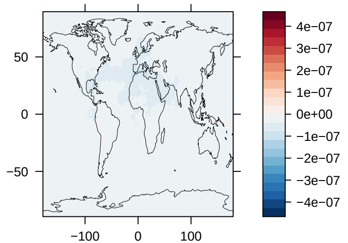
Load of SO 4 (% Diff) – NorESM2
