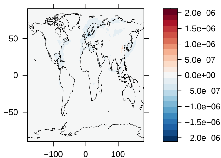
Load of SO 2 (kg/m 2 ) – GFDL-ESM4
