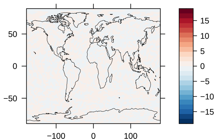
Upwelling Longwave Radiation at TOA (% Diff) – E3SM
