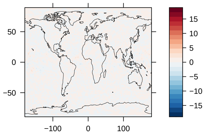
Clear-Sky Upwelling Shortwave Radiation at TOA (% Diff) – NorESM2
