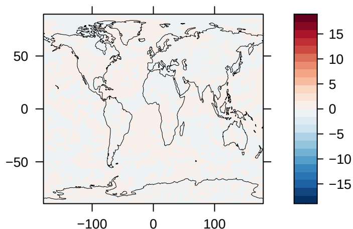
Clear-Sky Upwelling Longwave Radiation at TOA (% Diff) – E3SM
