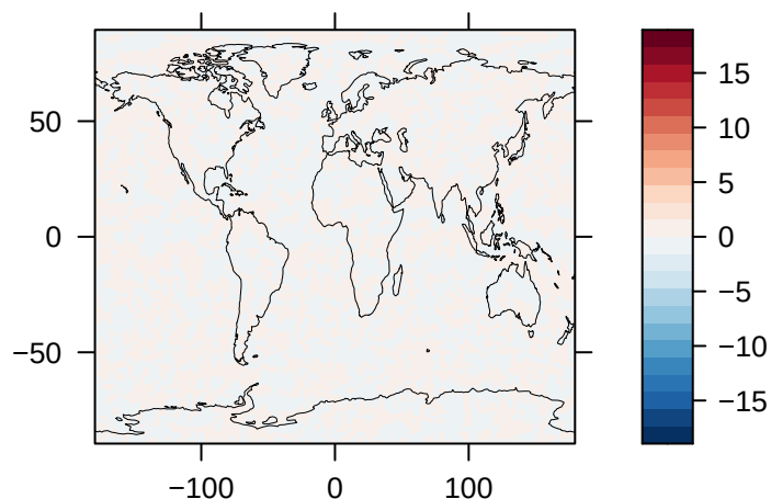
Upwelling Longwave Radiation at TOA (% Diff) – CAM-ATRAS
