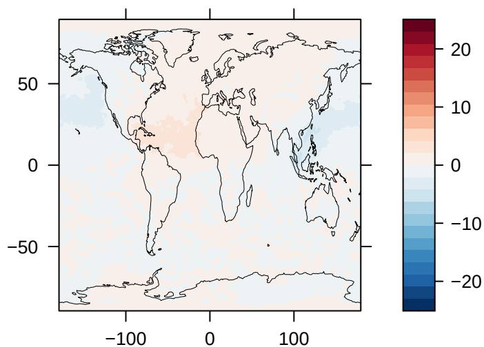
Load of SO4 (% Diff) – GFDL-ESM4
