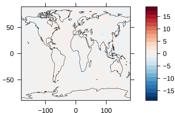
Upwelling Shortwave Radiation at TOA (% Diff) – CESM1
