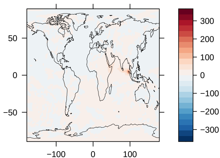
Load of SO2 (% Diff) – CESM1
