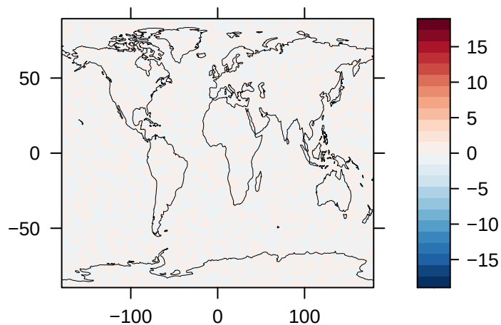
Upwelling Longwave Radiation at TOA (% Diff) – GISS-E2.1
