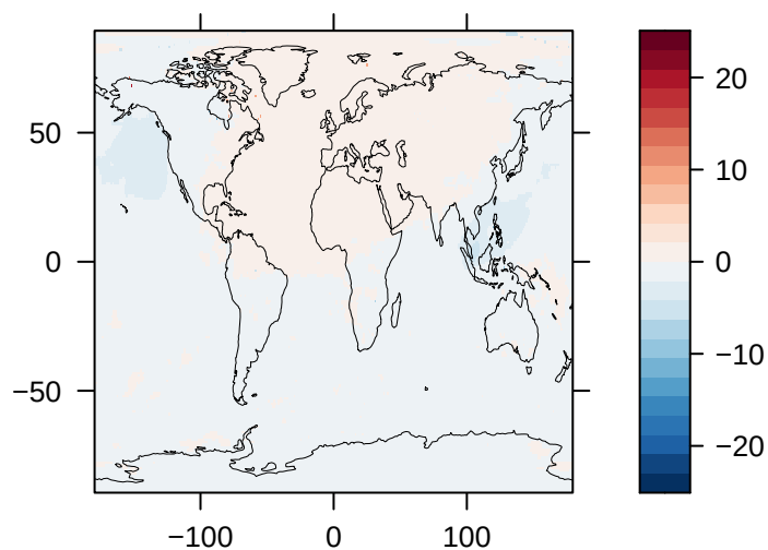
Load of SO4 (% Diff) – E3SM
