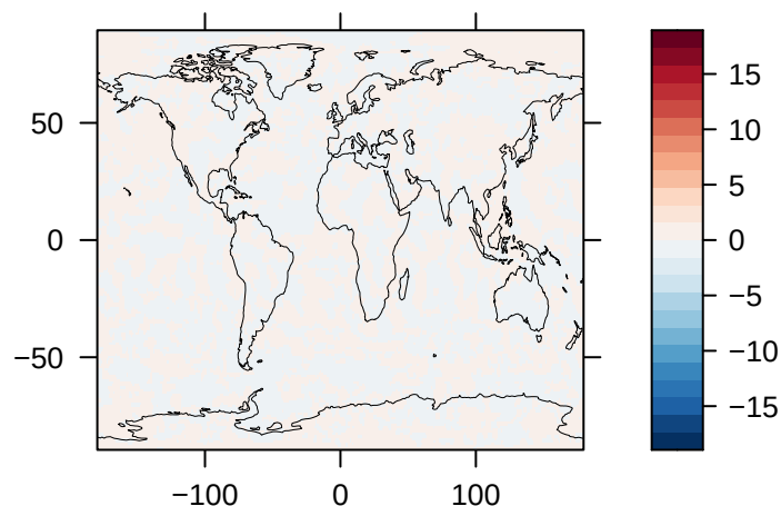
Upwelling Longwave Radiation at TOA (% Diff) – CESM1
