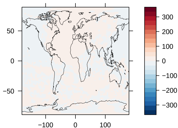
Load of SO2 (% Diff) – E3SM
