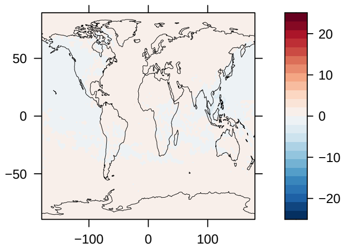
Load of SO4 (% Diff) – NorESM2
