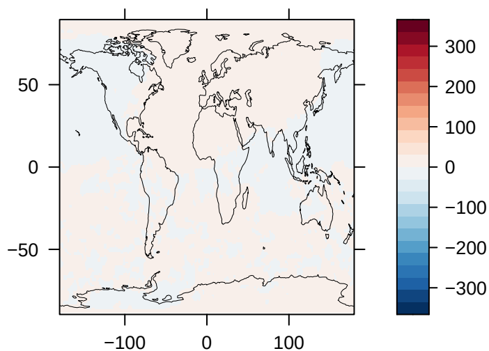
Load of SO2 (% Diff) – GISS-E2.1
