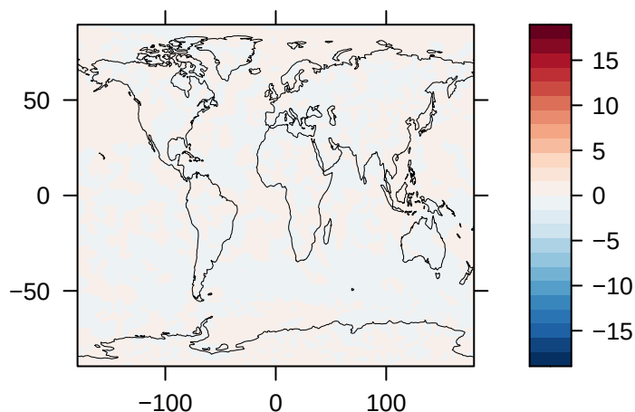
Clear-Sky Upwelling Longwave Radiation at TOA (% Diff) – CESM1
