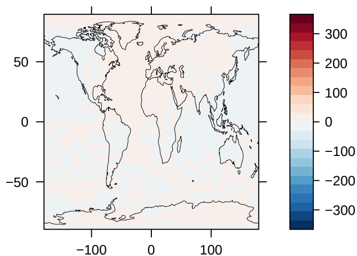
Load of SO2 (% Diff) – CAM-ATRAS
