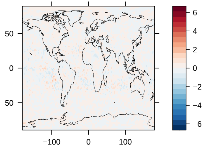
Cloud Area Fraction (% Diff) – CAM-ATRAS
