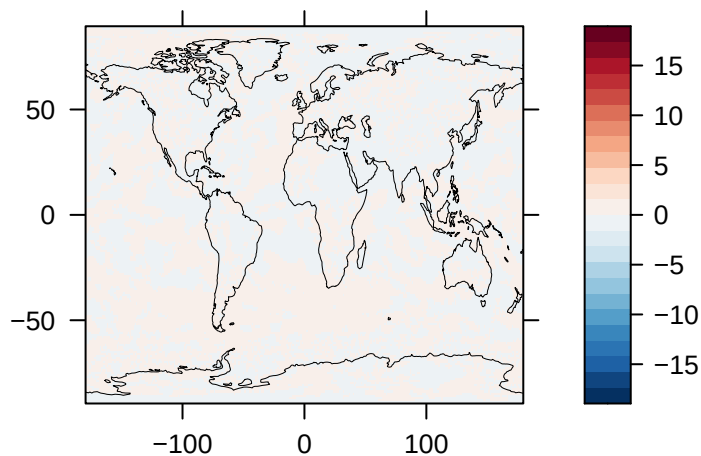
Clear-Sky Upwelling Longwave Radiation at TOA (% Diff) – NorESM2
