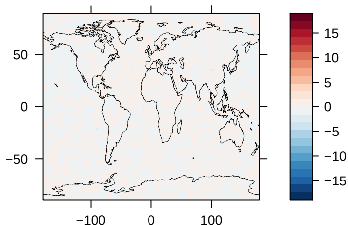
Upwelling Clear-Sky Longwave Radiation at TOA (% Diff) – CAM-ATRAS
