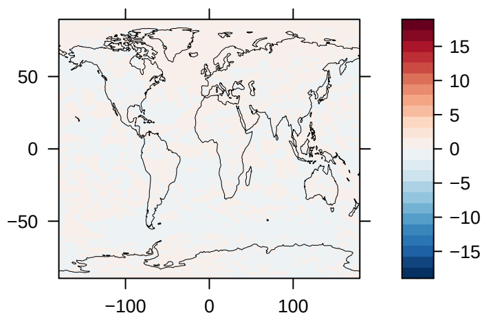
Clear-Sky Upwelling Longwave Radiation at TOA (% Diff) – GFDL-ESM4
