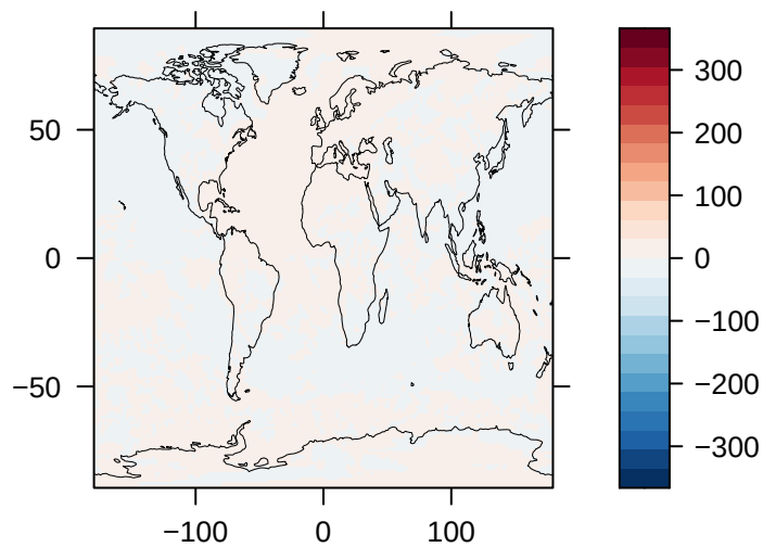
Load of SO2 (% Diff) – NorESM2
