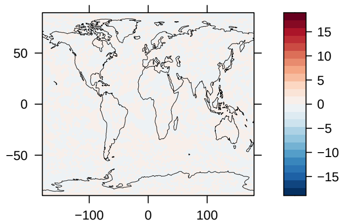
Upwelling Longwave Radiation at TOA (% Diff) – NorESM2
