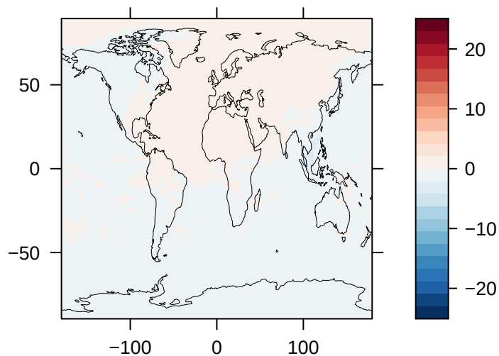
Load of SO4 (% Diff) – GISS-E2.1
