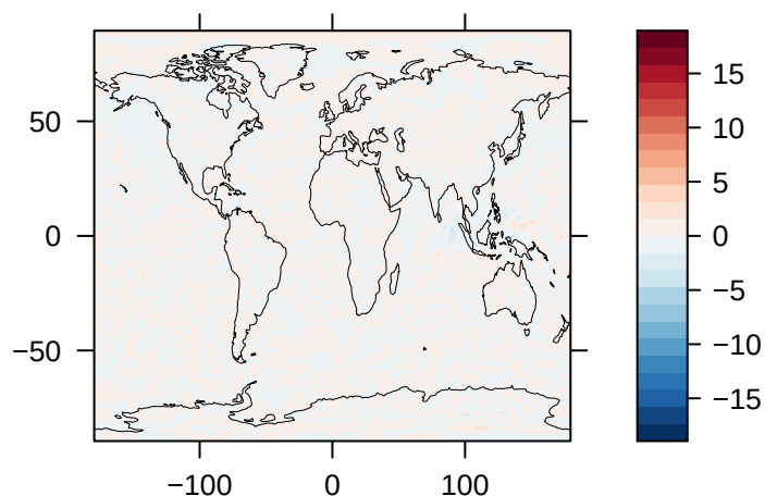
Upwelling Shortwave Radiation at TOA (% Diff) – E3SM
