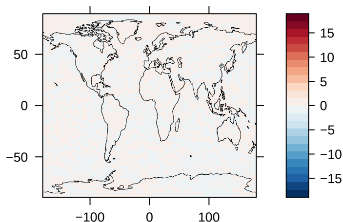
Upwelling Longwave Radiation at TOA (% Diff) – GFDL-ESM4
