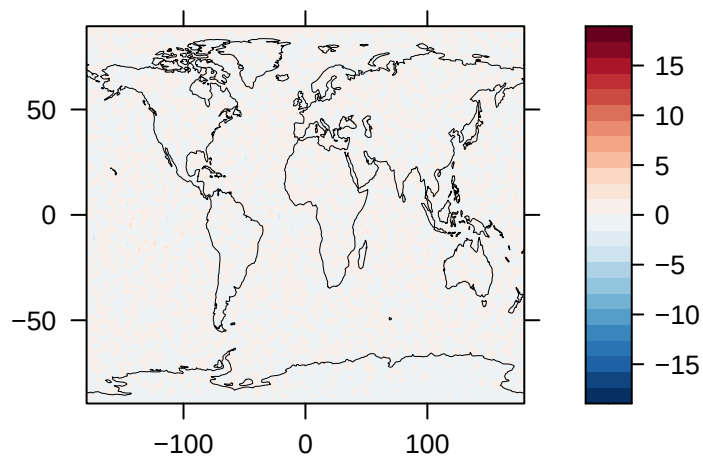
Clear-Sky Upwelling Shortwave Radiation at TOA (% Diff) – GISS-E2.1
