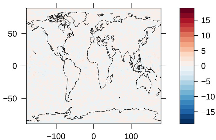
Upwelling Shortwave Radiation at TOA (% Diff) – NorESM2
