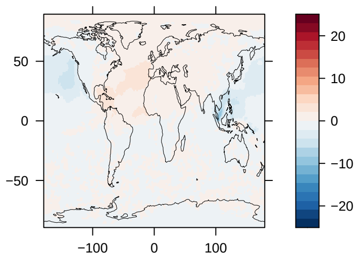
Load of SO4 (% Diff) – CAM-ATRAS
