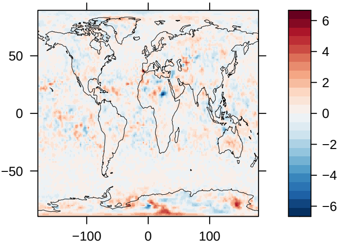
Cloud Area Fraction (% Diff) – CESM1
