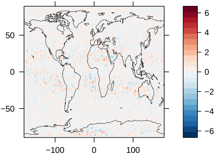
Cloud Area Fraction (% Diff) – GISS-E2.1
