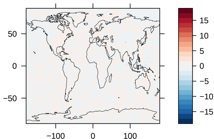
Clear-Sky Upwelling Shortwave Radiation at TOA (% Diff) – CESM1
