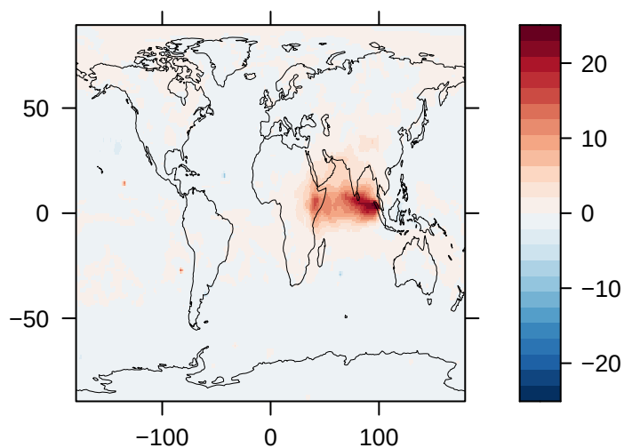
Load of SO4 (% Diff) – CESM1
