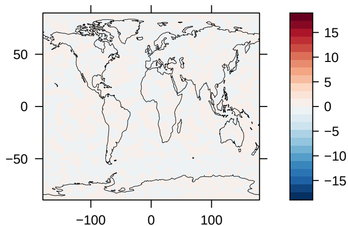
Clear-Sky Upwelling Longwave Radiation at TOA (% Diff) – GISS-E2.1
