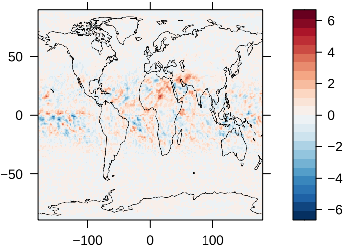
Cloud Area Fraction (% Diff) – NorESM2
