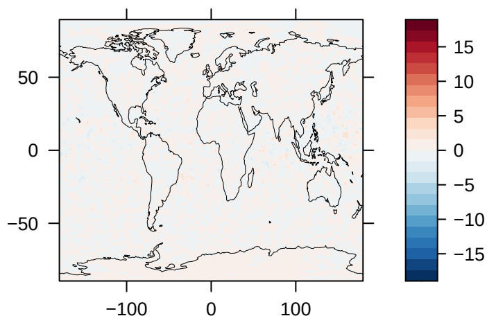
Upwelling Shortwave Radiation at TOA (% Diff) – GFDL-ESM4
