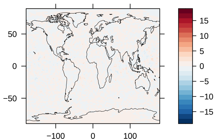
Clear-Sky Upwelling Shortwave Radiation at TOA (% Diff) – GFDL-ESM4
