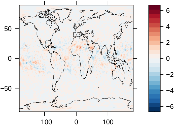
Cloud Area Fraction (% Diff) – E3SM
