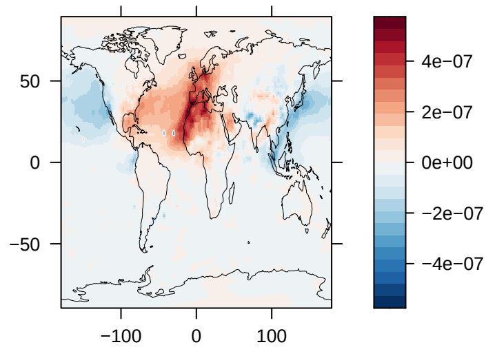
Load of SO4 (% Diff) – CESM1
