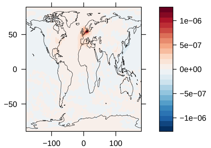
Load of SO2 (% Diff) – CESM1
