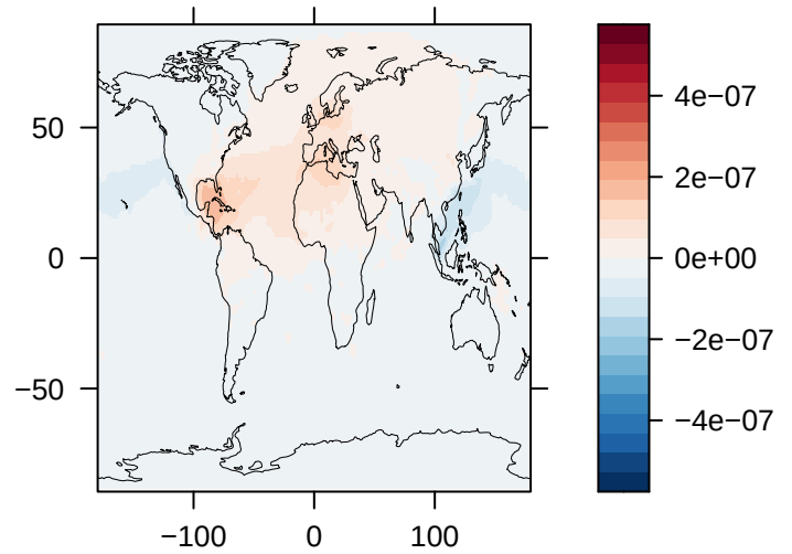
Load of SO4 (% Diff) – GISS-E2.1
