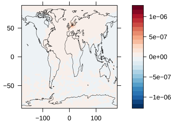
Load of SO2 (% Diff) – GISS-E2.1
