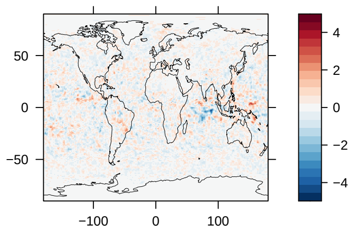
Clear-Sky Upwelling Shortwave Radiation at TOA (W/m 2 ) – GFDL-ESM4
