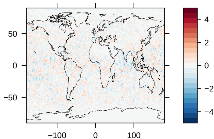
Clear-Sky Upwelling Shortwave Radiation at TOA (W/m 2 ) – GISS-E2.1
