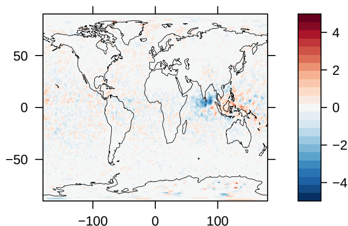
Clear-Sky Upwelling Shortwave Radiation at TOA (W/m 2 ) – E3SM
