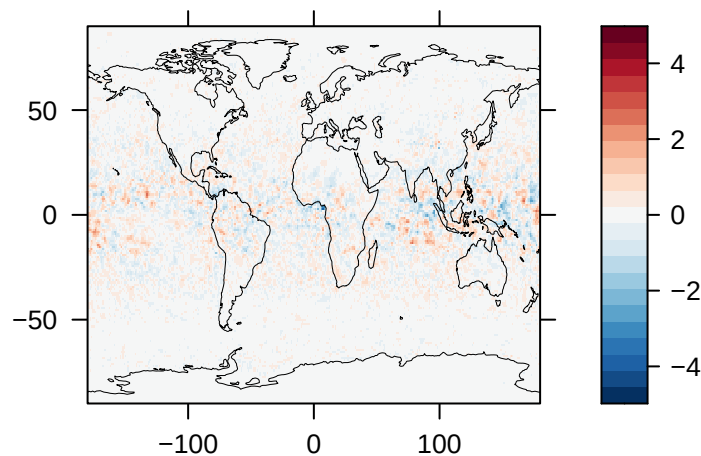
Clear-Sky Upwelling Shortwave Radiation at TOA (W/m 2 ) – NorESM2
