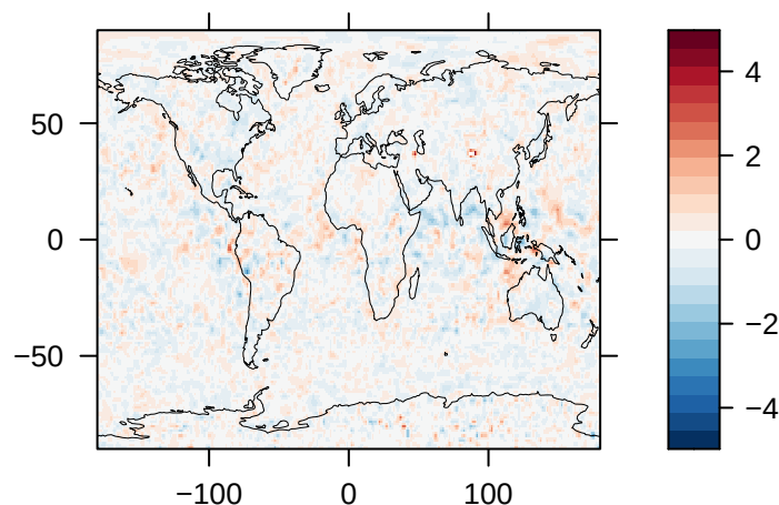
Clear-Sky Upwelling Shortwave Radiation at TOA (W/m 2 ) – CESM1
