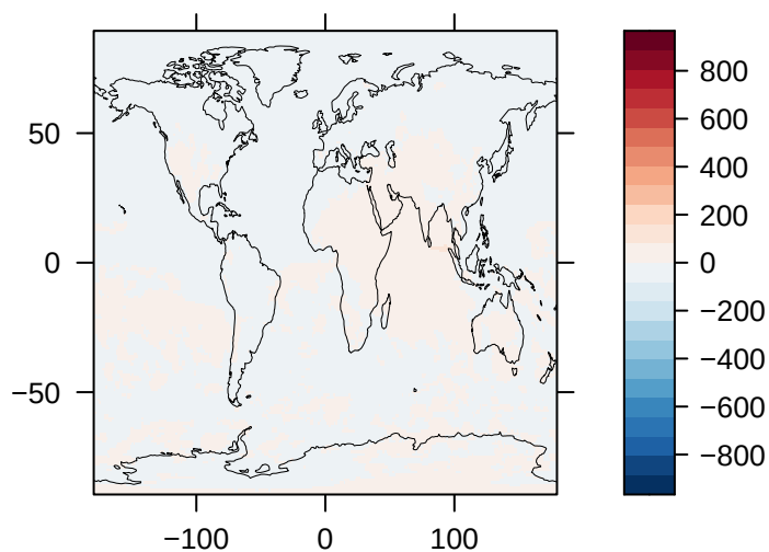
Load of SO2 (% Diff) – GFDL-ESM4
