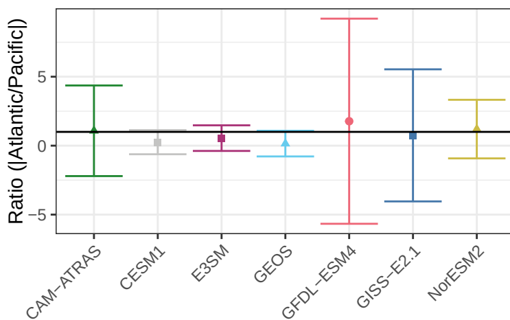
Clear-Sky Upwelling Longwave Flux – Ratio Between Atlantic and Pacific
