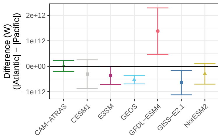
Clear-Sky Upwelling Shortwave Flux – Difference Between Atlantic and Pacific
