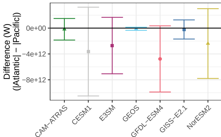
Upwelling Longwave Flux – Difference Between Atlantic and Pacific
