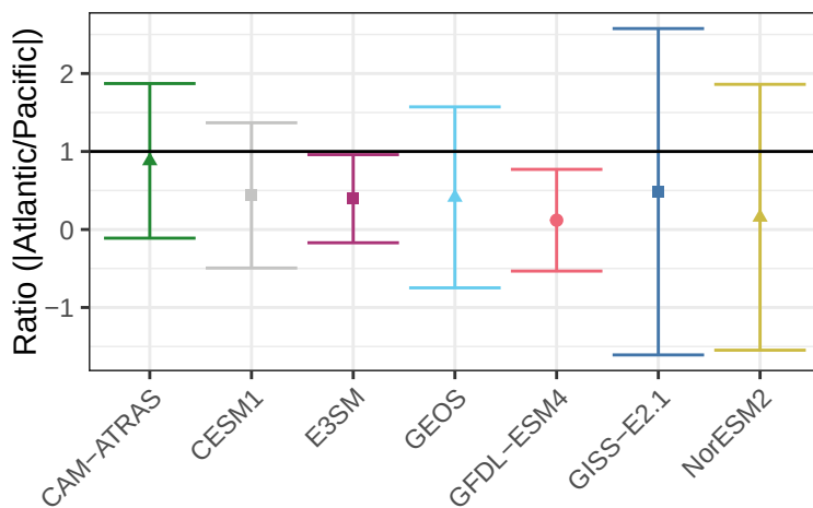
Upwelling Longwave Flux – Ratio Between Atlantic and Pacific
