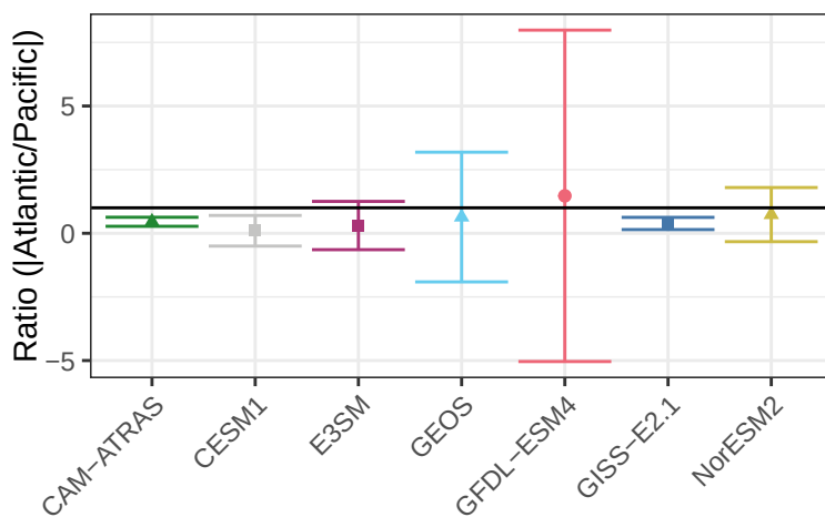
Implied Cloud Response – Ratio Between Atlantic and Pacific
