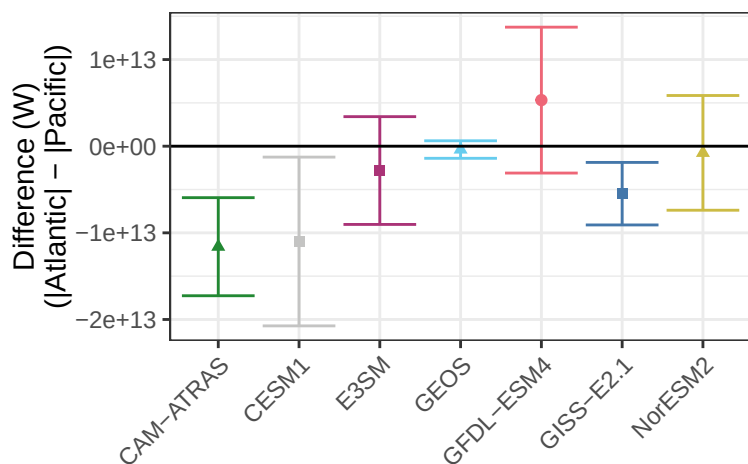
Net Radiative Flux – Difference Between Atlantic and Pacific
