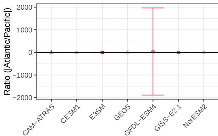
Net Radiative Flux – Ratio Between Atlantic and Pacific
