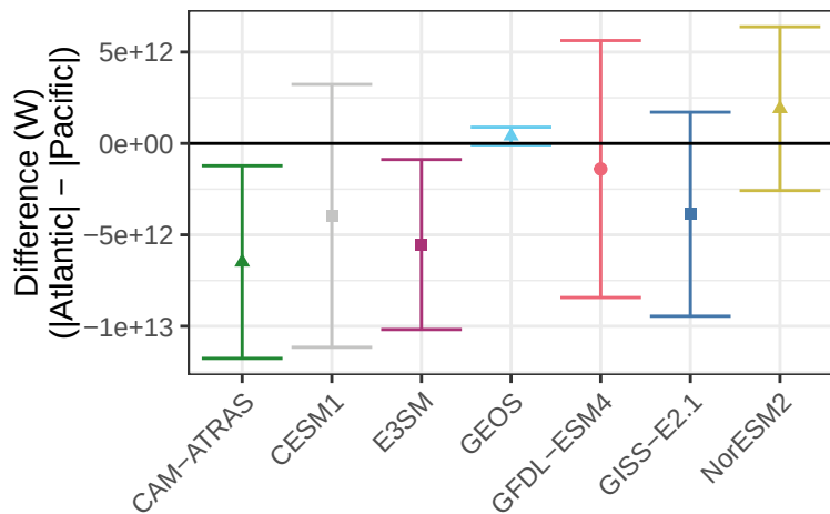
Upwelling Shortwave Flux – Difference Between Atlantic and Pacific
