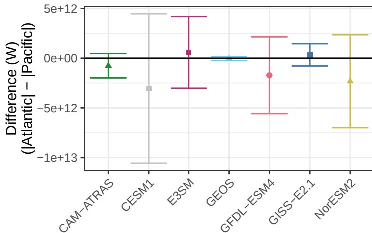
Upwelling Longwave Flux – Difference Between Atlantic and Pacific
