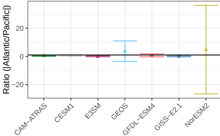
Upwelling Shortwave Flux – Ratio Between Atlantic and Pacific
