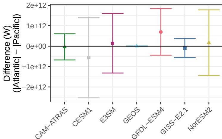
Clear-Sky Upwelling Longwave Flux – Difference Between Atlantic and Pacific
