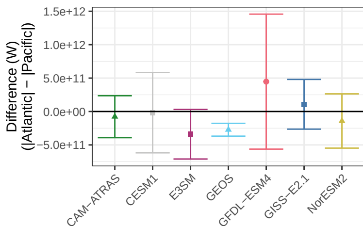
Clear-Sky Upwelling Shortwave Flux Difference Between Atlantic and Pacific
