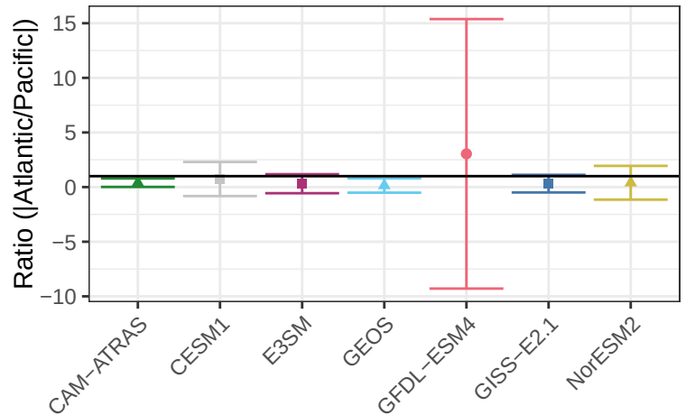
Implied Cloud Response – Ratio Between Atlantic and Pacific
