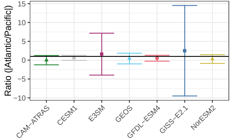
Upwelling Longwave Flux – Ratio Between Atlantic and Pacific
