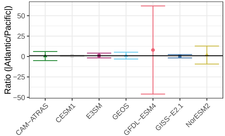
Clear-Sky Upwelling Longwave Flux – Ratio Between Atlantic and Pacific
