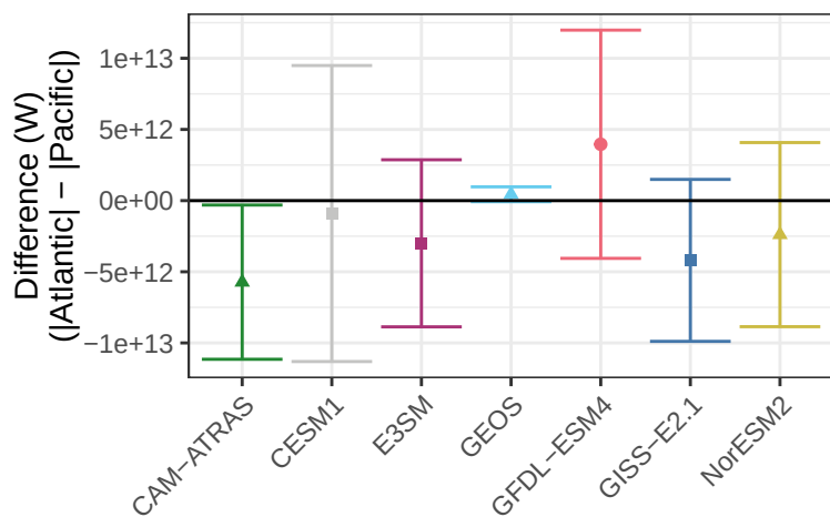
Net Radiative Flux – Difference Between Atlantic and Pacific
