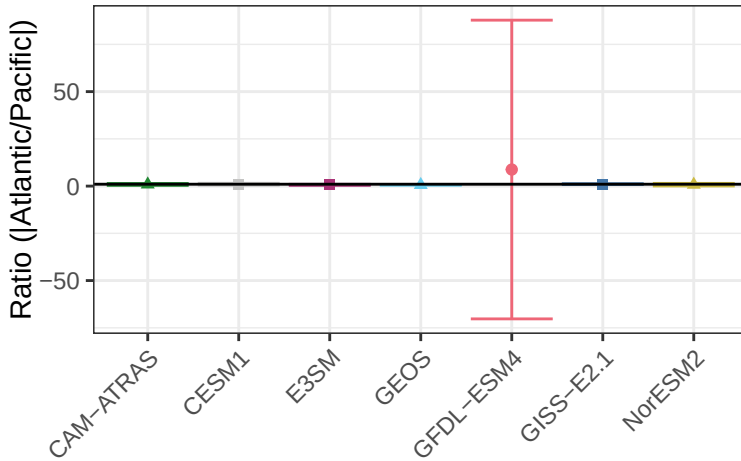
Clear-Sky Upwelling Shortwave Flux – Ratio Between Atlantic and Pacific
