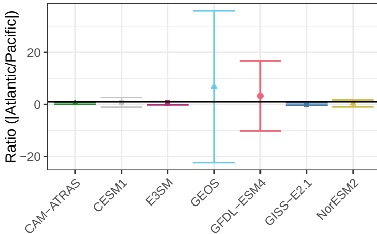
Net Radiative Flux – Ratio Between Atlantic and Pacific
