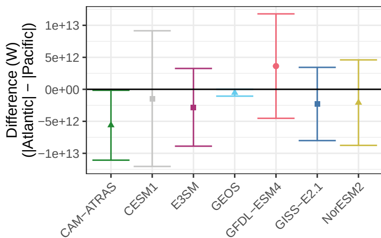
Implied Cloud Response – Difference Between Atlantic and Pacific
