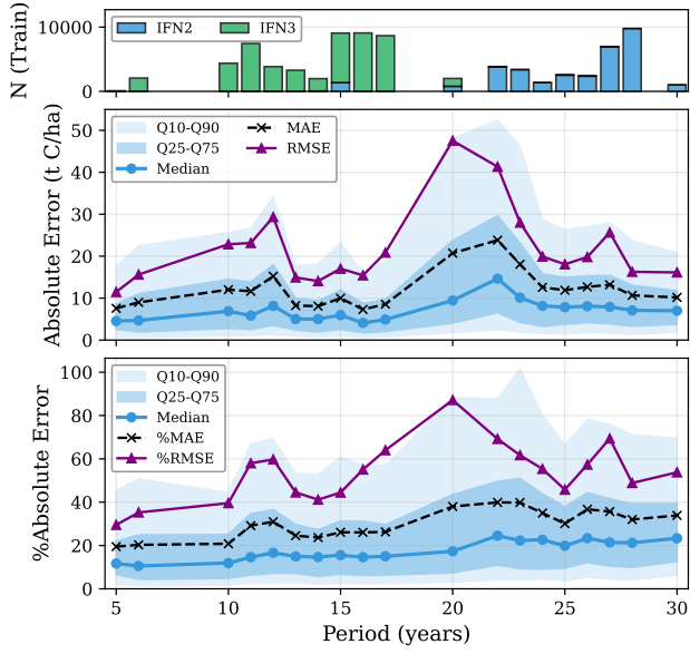
(a) LightGBM global , c4 (tC/ha).
