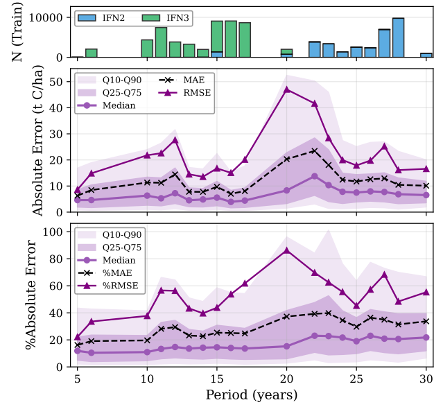
(b) Stacking global (Conf. 5, MLP), c4 (tC/ha).
