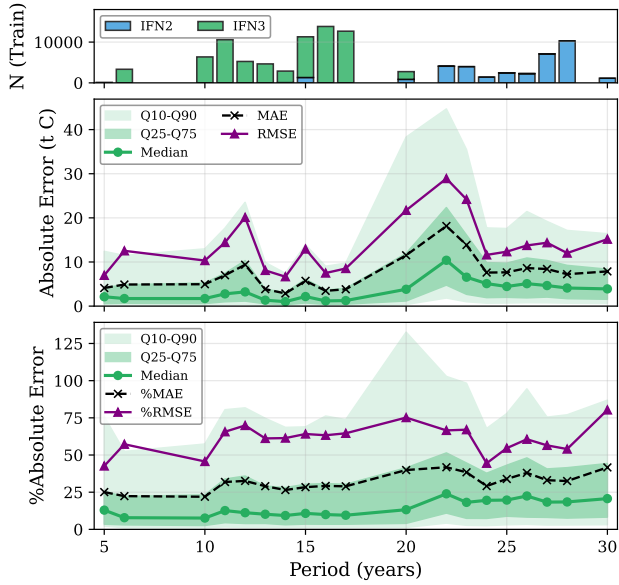
(c) CatBoost global , carbono_bruto4 (tC).
