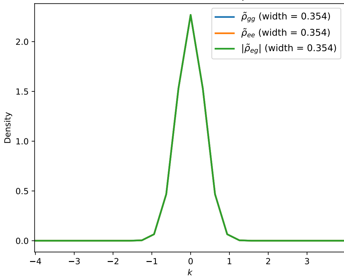
Initial State (Momentum Space)
