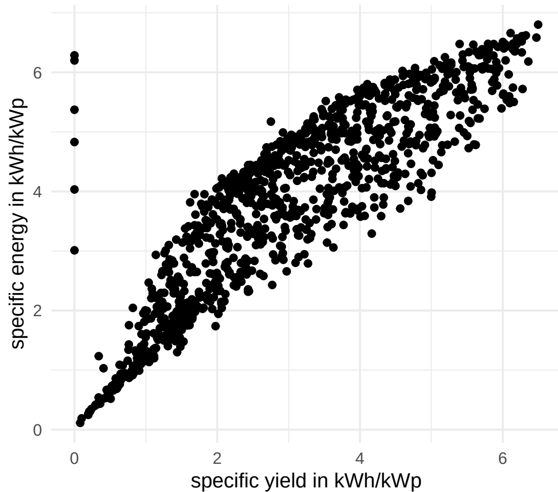
household 96 vs. household 159
