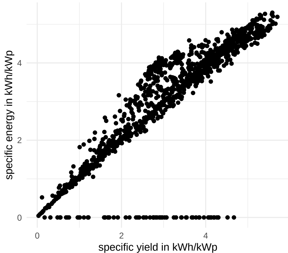
household 40 vs. household 99
