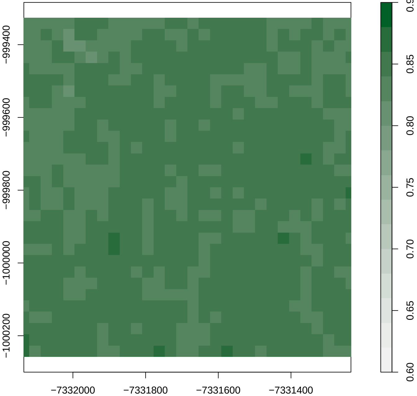
NDVI | 2016-10-20 P1D
