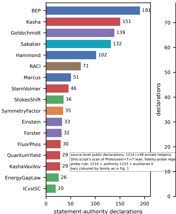
(a) scale: 1153 statement-authority declarations over 92 theory modules
