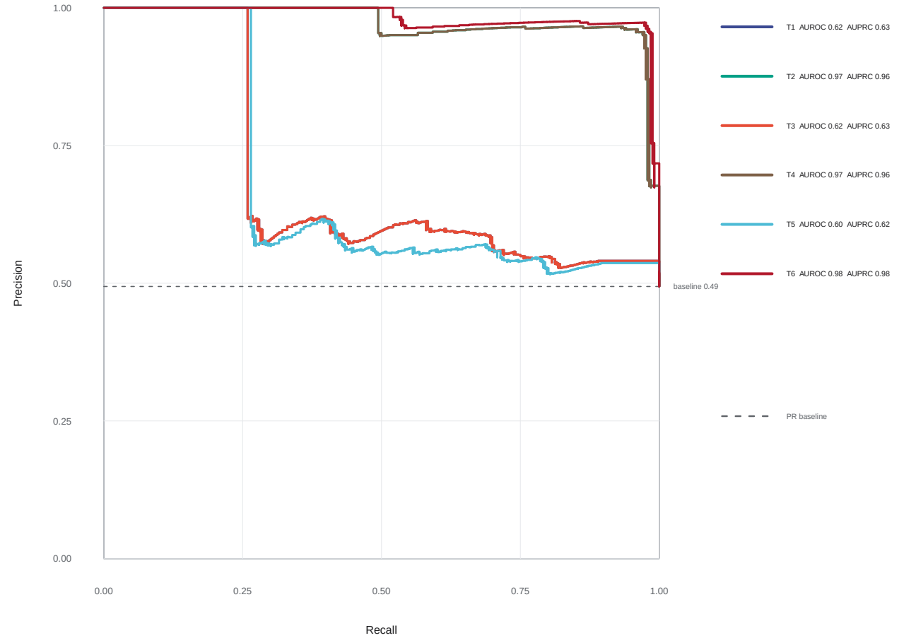
PR; median AUPRC = 0.797
