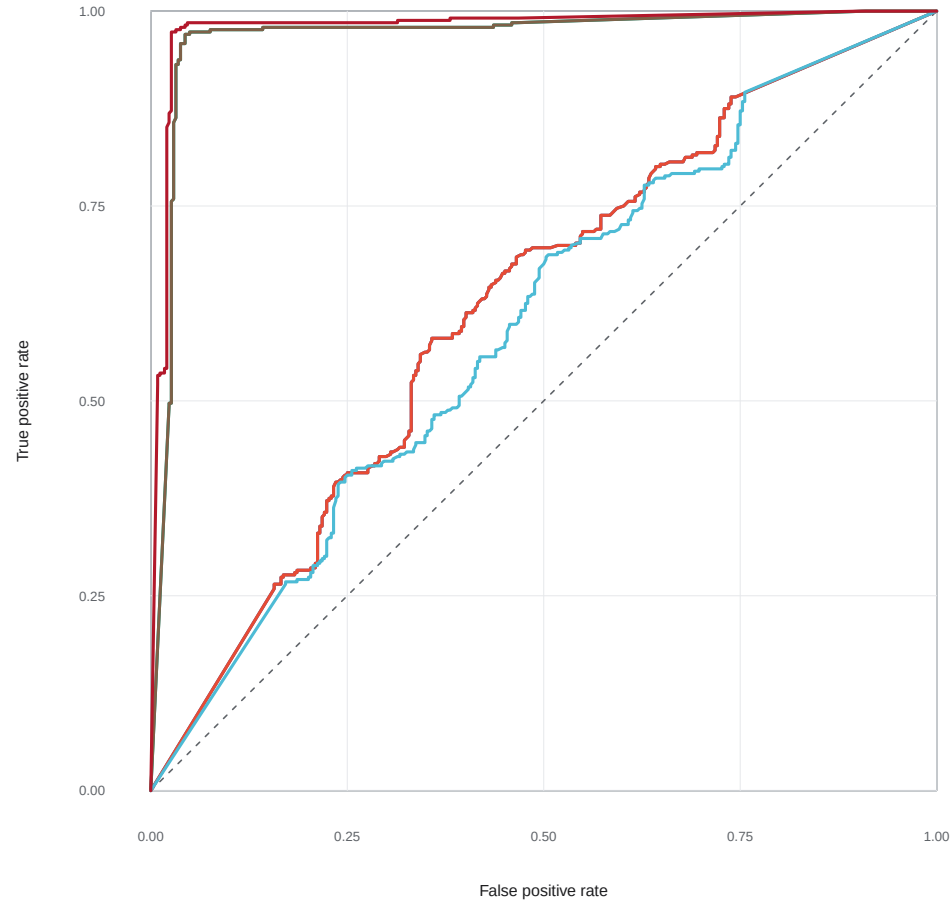
ROC; median AUROC = 0.793
