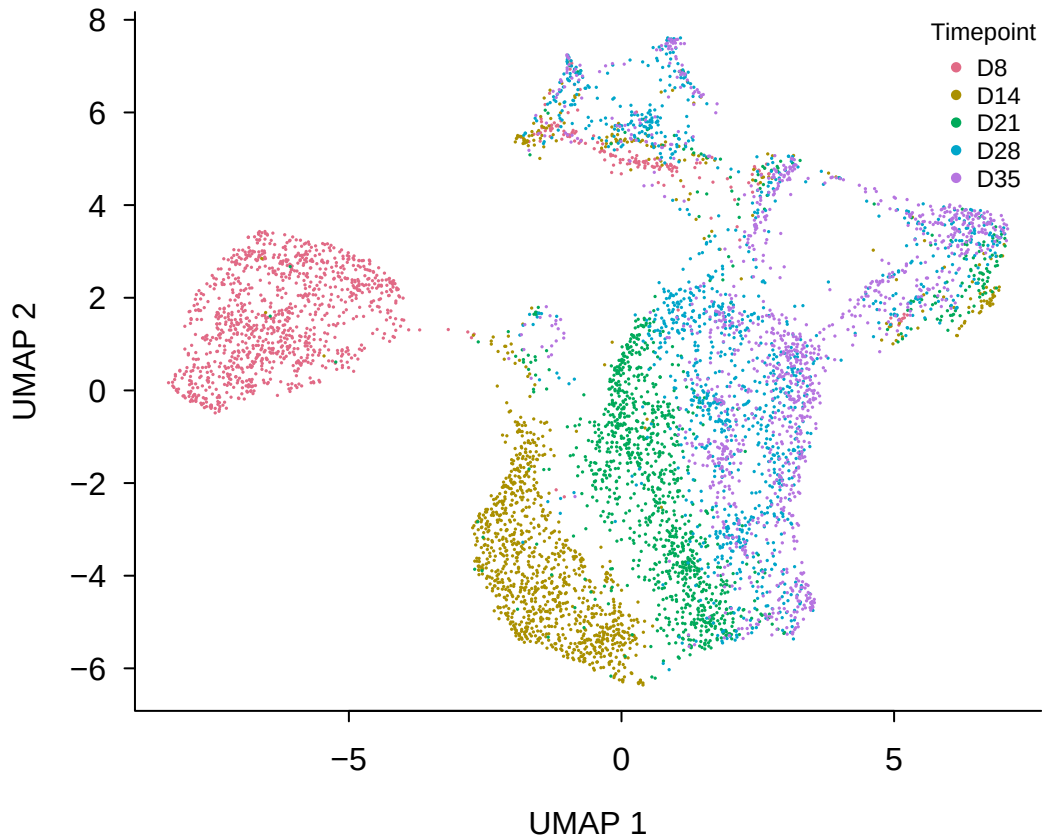
GSE204796 time-course cell-state layout
