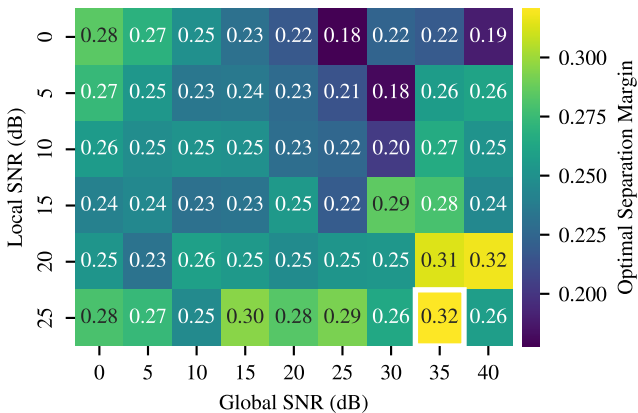
DeepBeat
