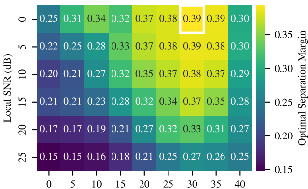
DeepBeat
