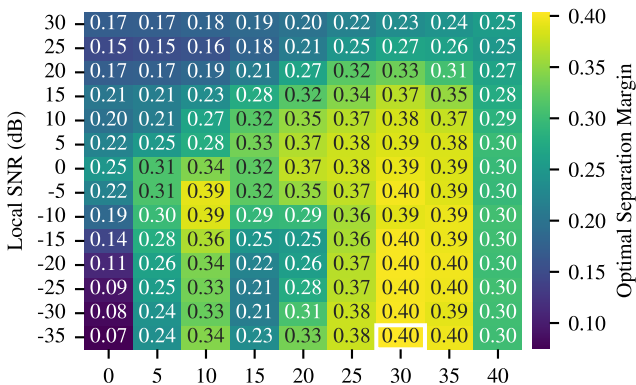
DeepBeat
