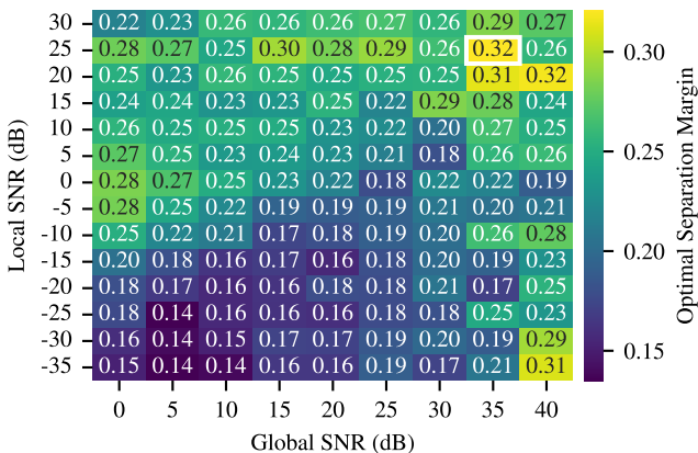
DeepBeat
