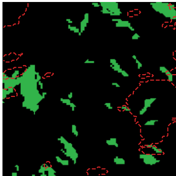
GT + TGD
