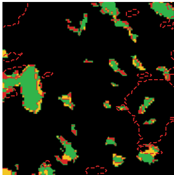
SO errors
