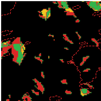
MFEWF errors
