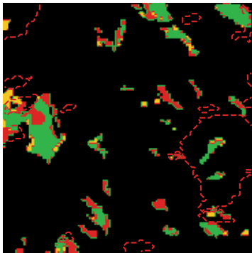
Boehm errors
