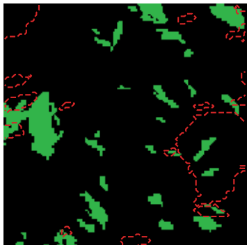
GT + TGD
