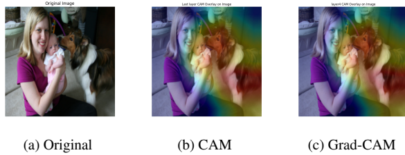
Figure 4. Visualization of class-discriminative regions for a correctly classified sample from the Stanford Dogs dataset. (a) Original input image. (b) CAM-based activation map overlaid on the image. (c) Grad-CAM activation map for the same model and class, showing qualitatively similar localization behavior.
