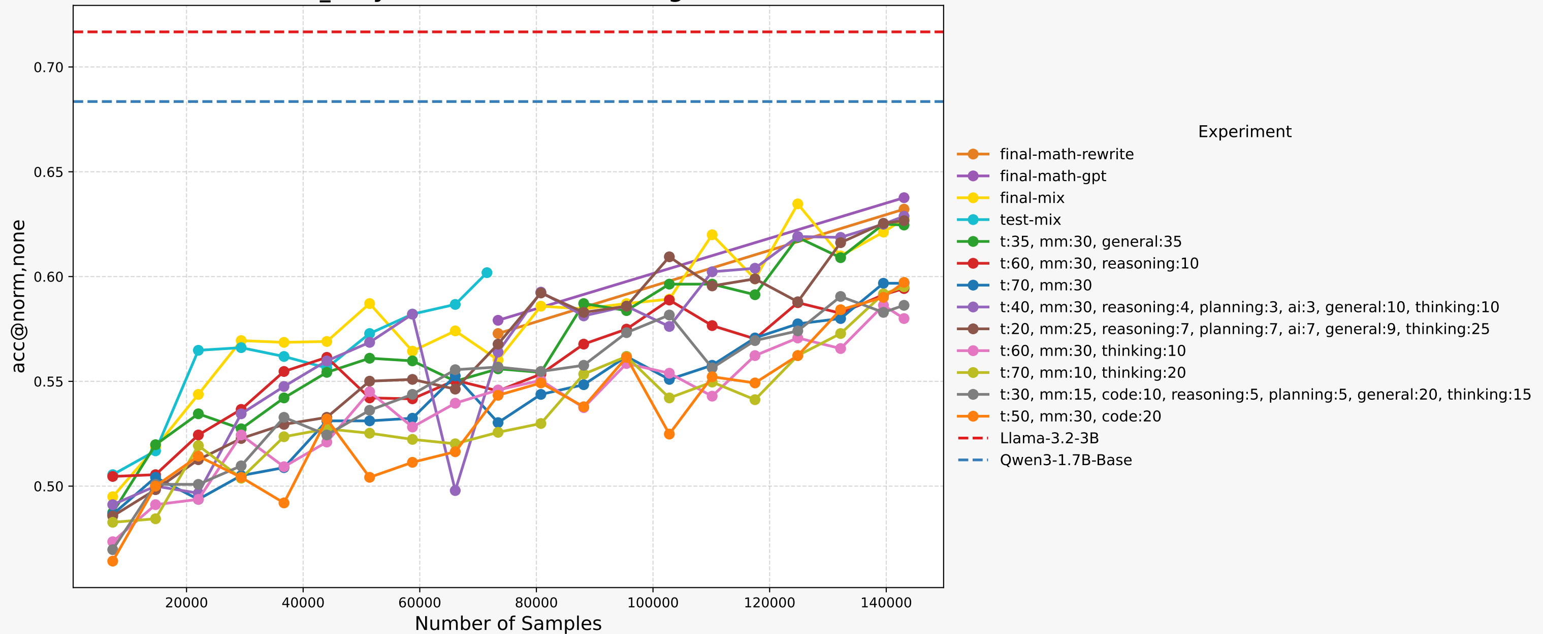
arc_easy Tokenmix Ablation Progress
