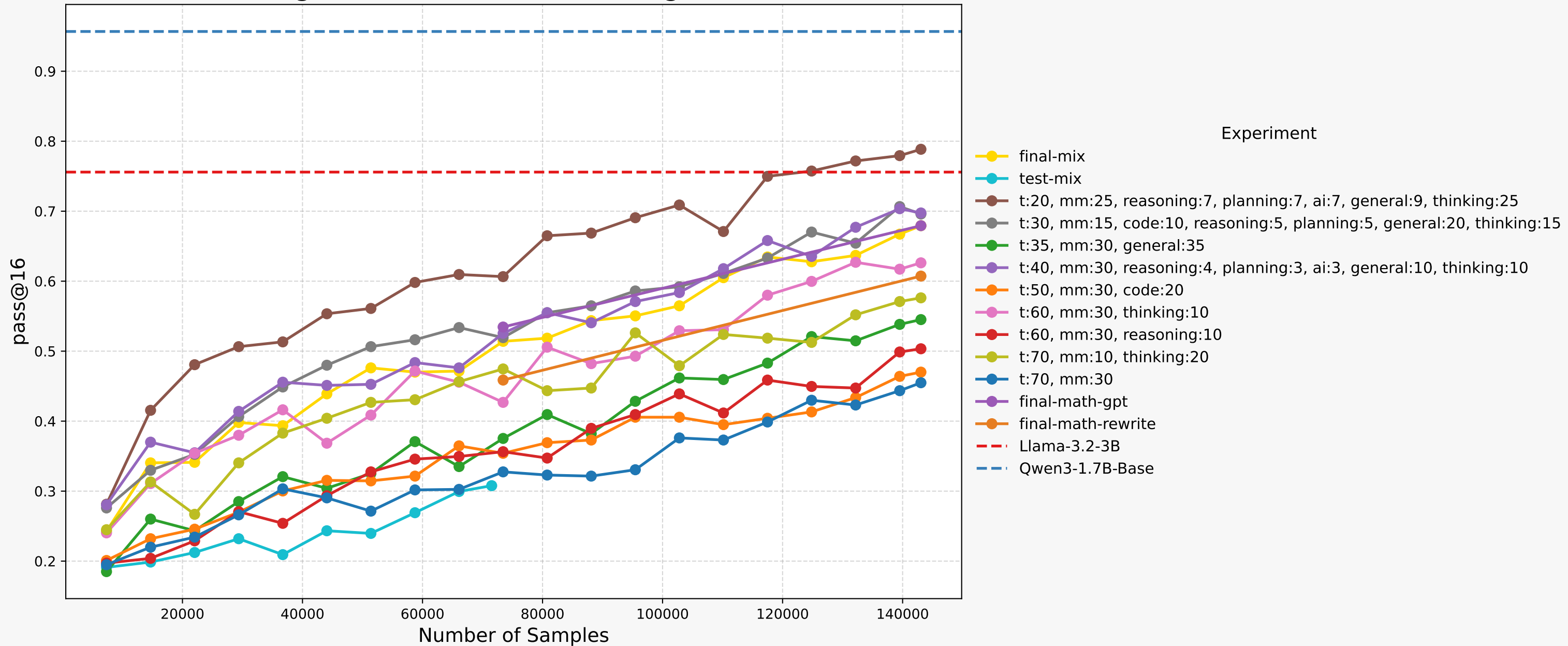
gsm8k Tokenmix Ablation Progress
