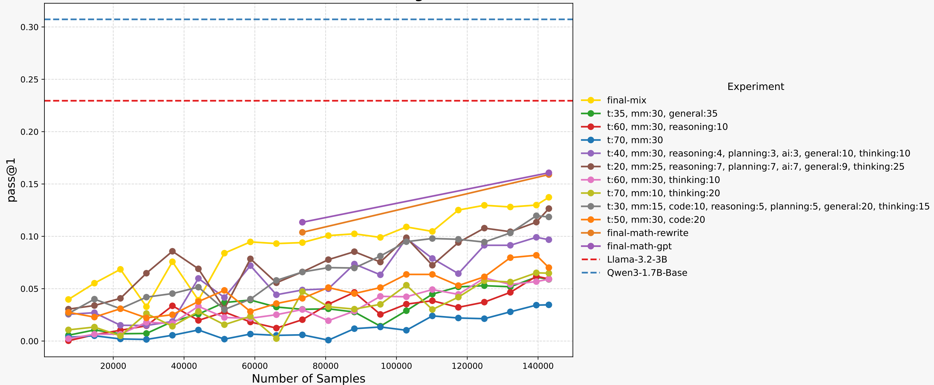
humaneval Tokenmix Ablation Progress
