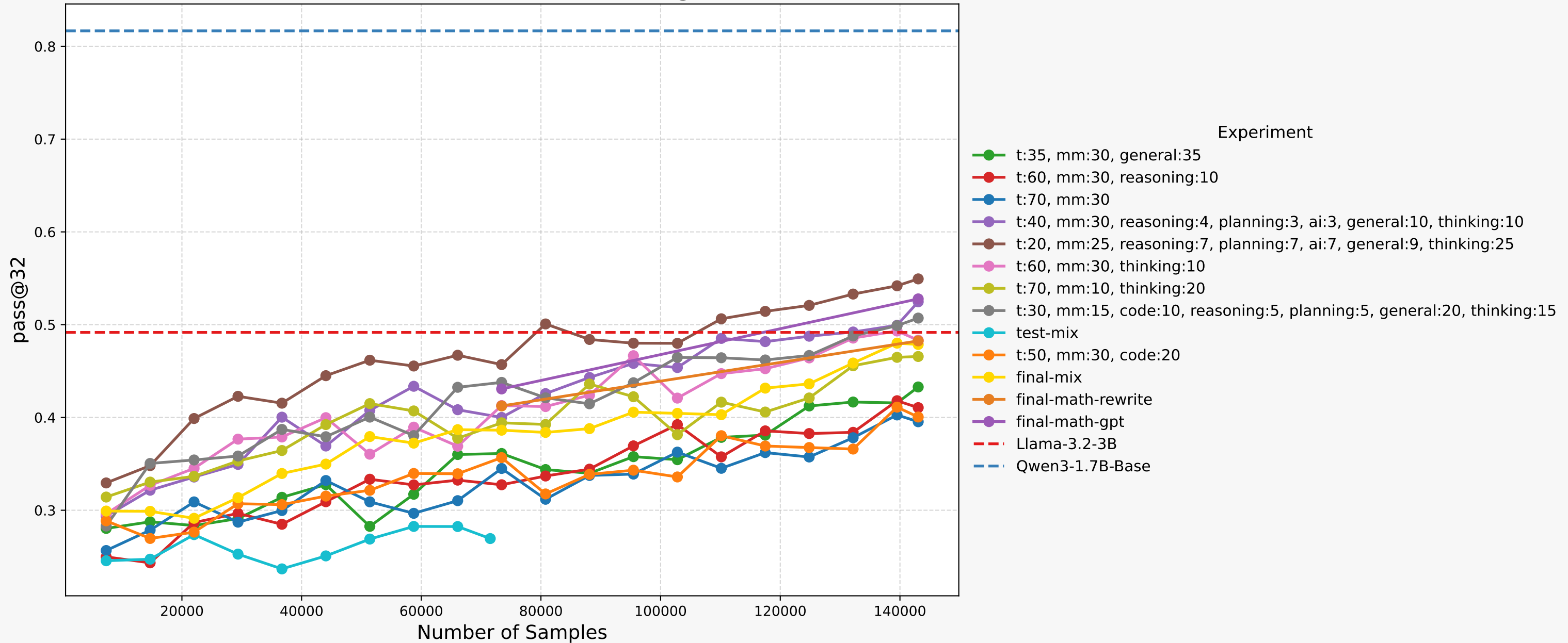
math500 Tokenmix Ablation Progress
