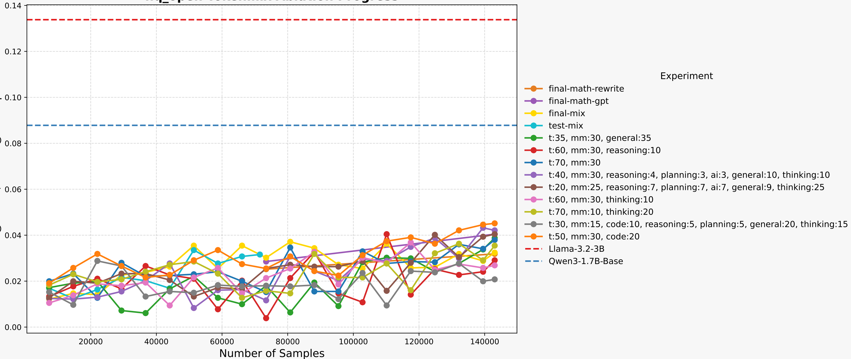
nq_open Tokenmix Ablation Progress
